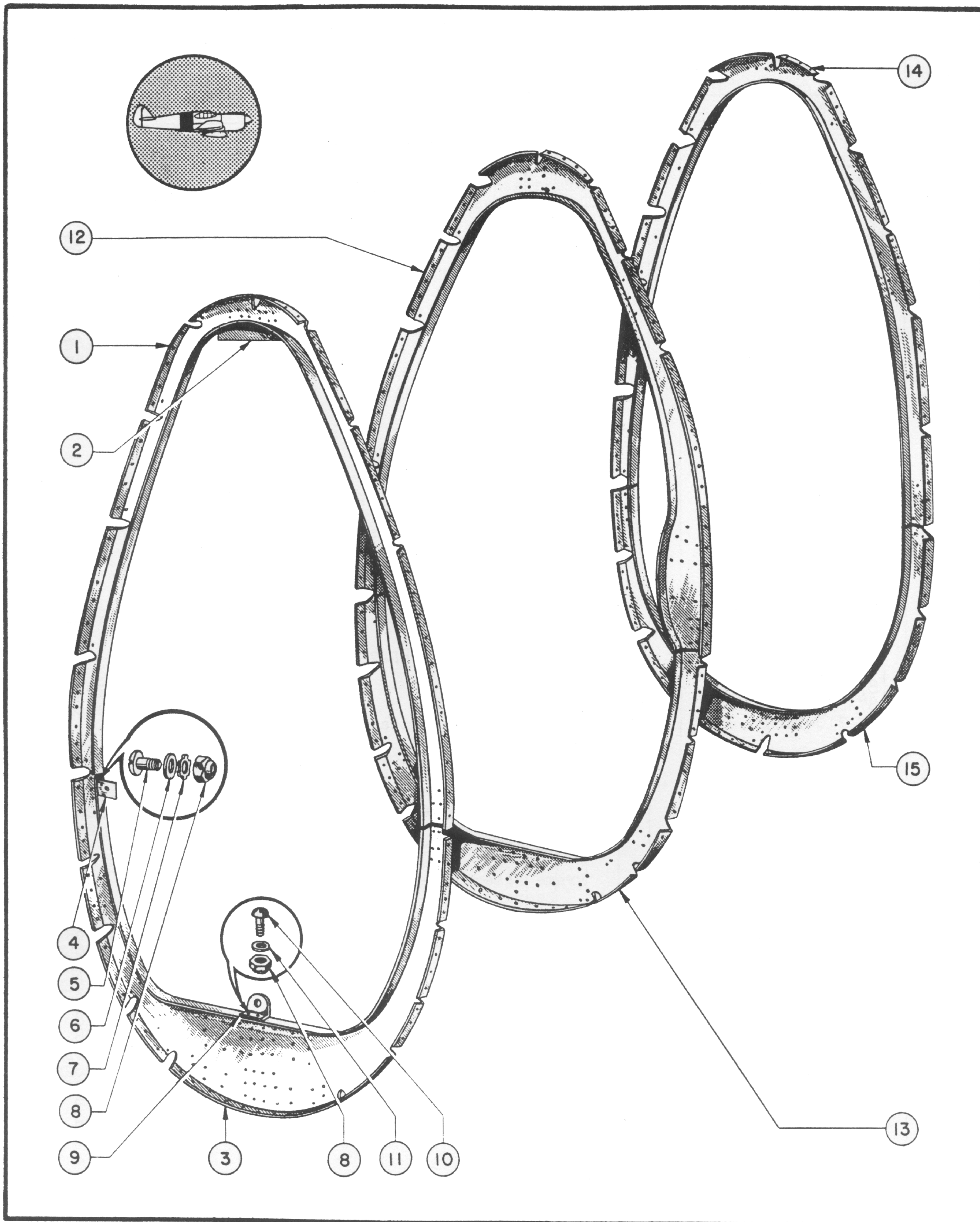
Figure 29—Bulkhead Assemblies Stations 9, 10, and 11
