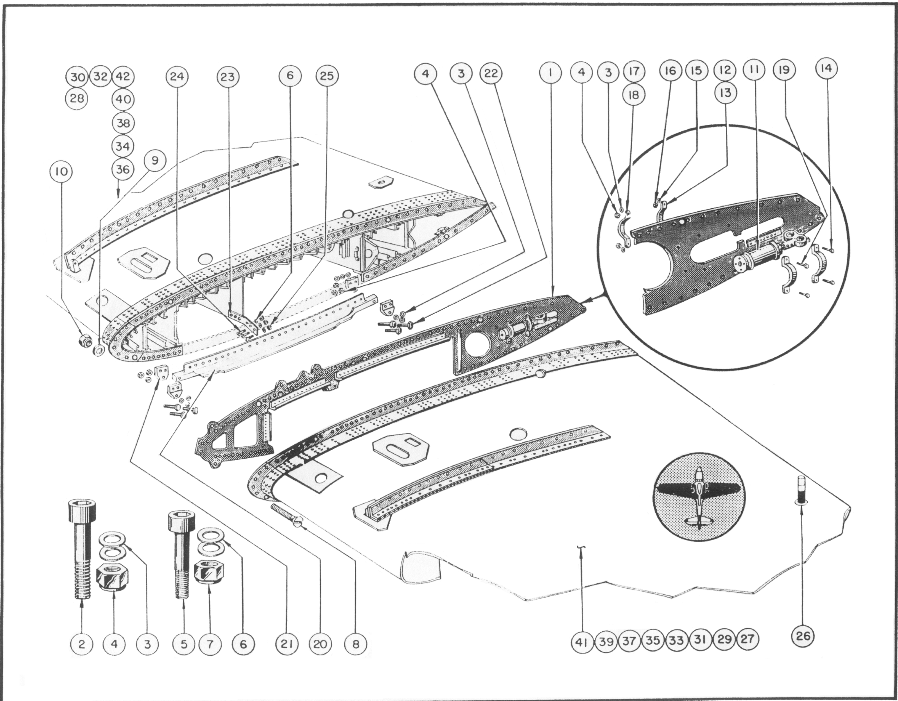
Figure 3—Wing Erection
