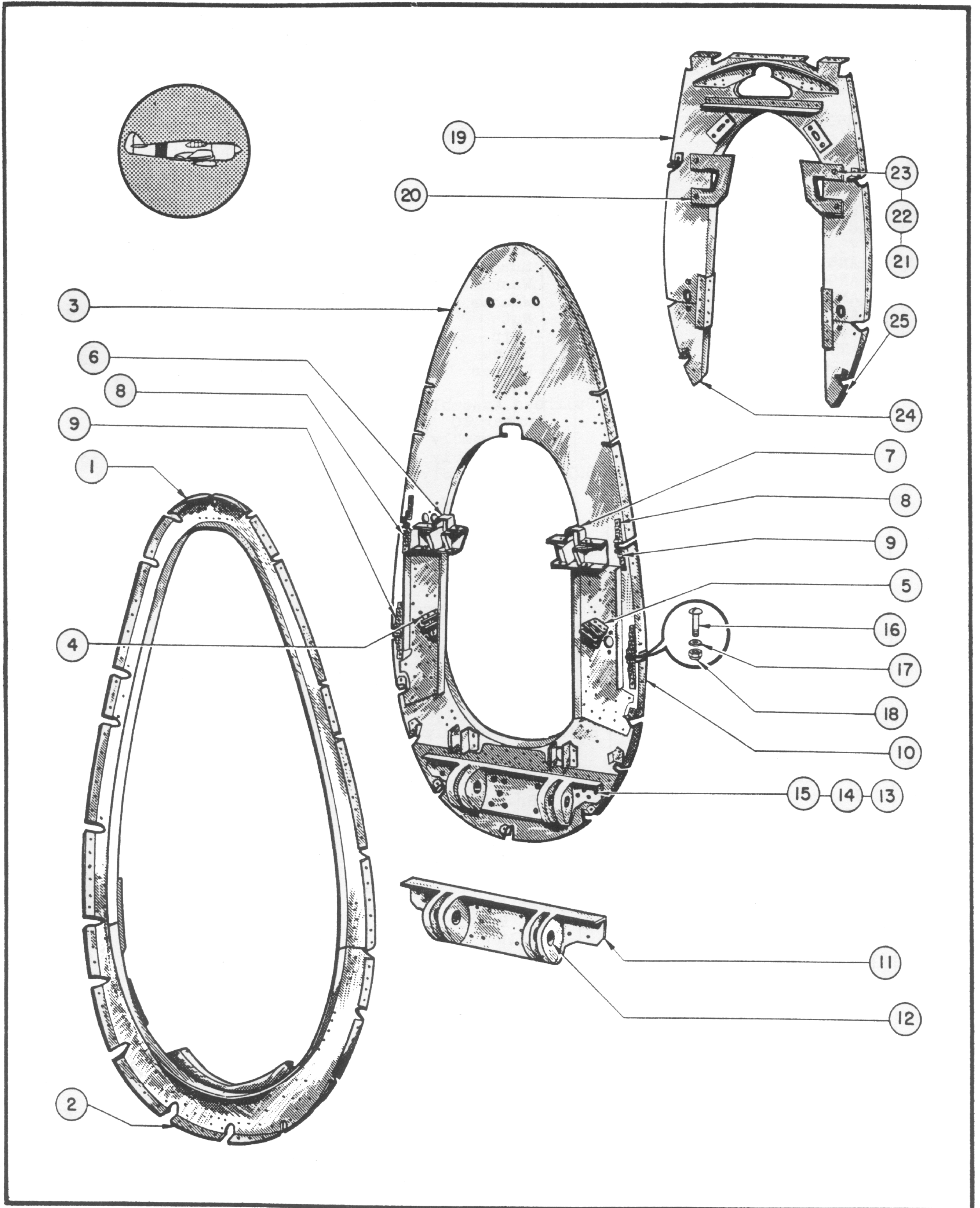
Figure 30—Bulkhead Assemblies Stations 12, 13, and 14
