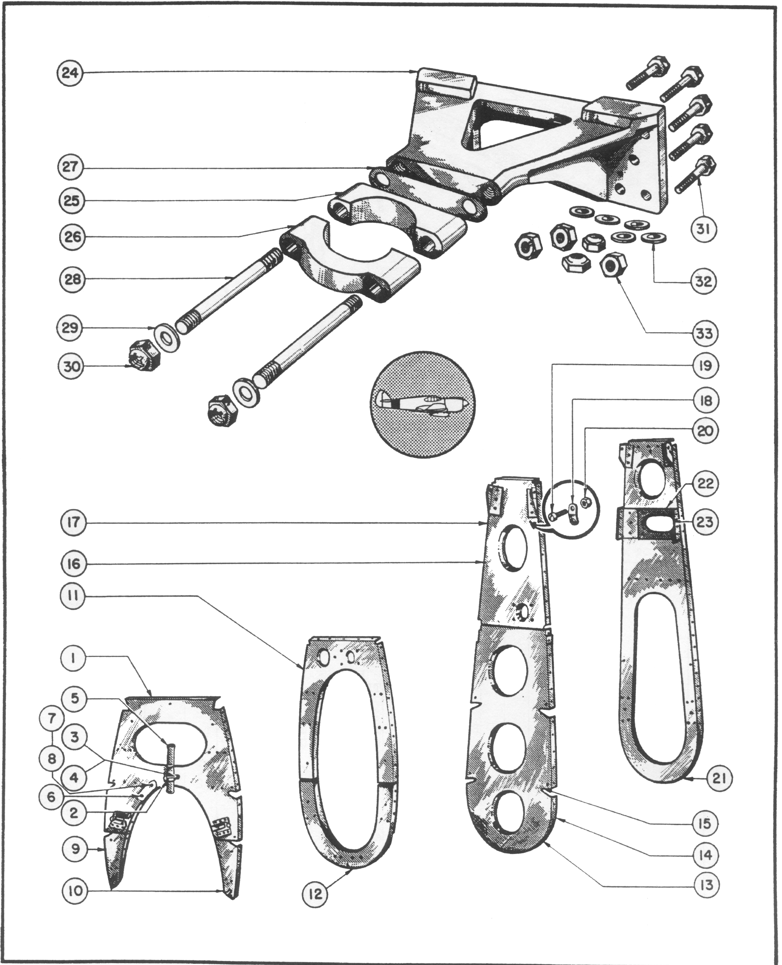
Figure 31—Bulkhead Assemblies Stations 15, 16, 17, and 18
