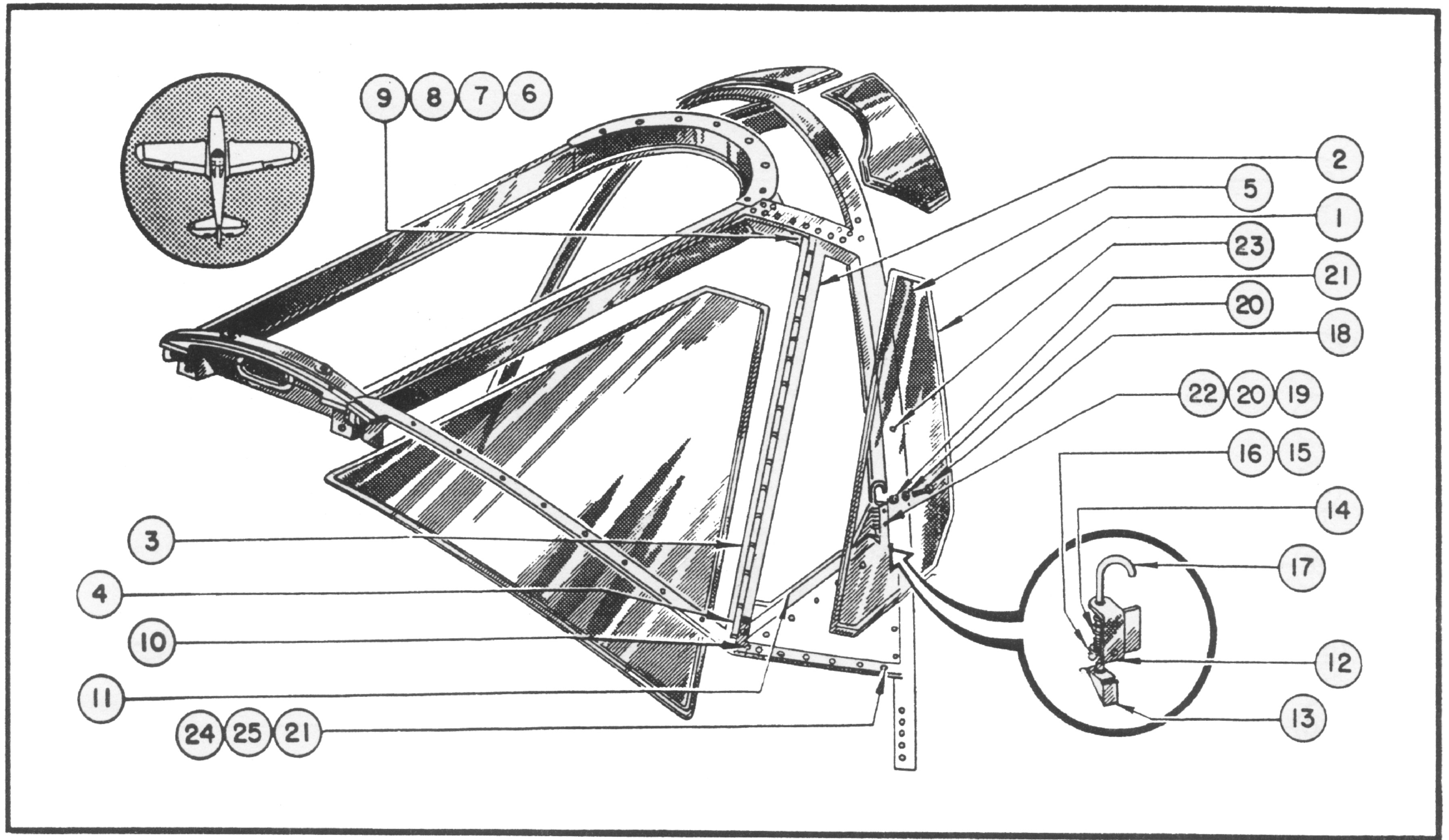
Figure 32—Windshield Panel Installation
