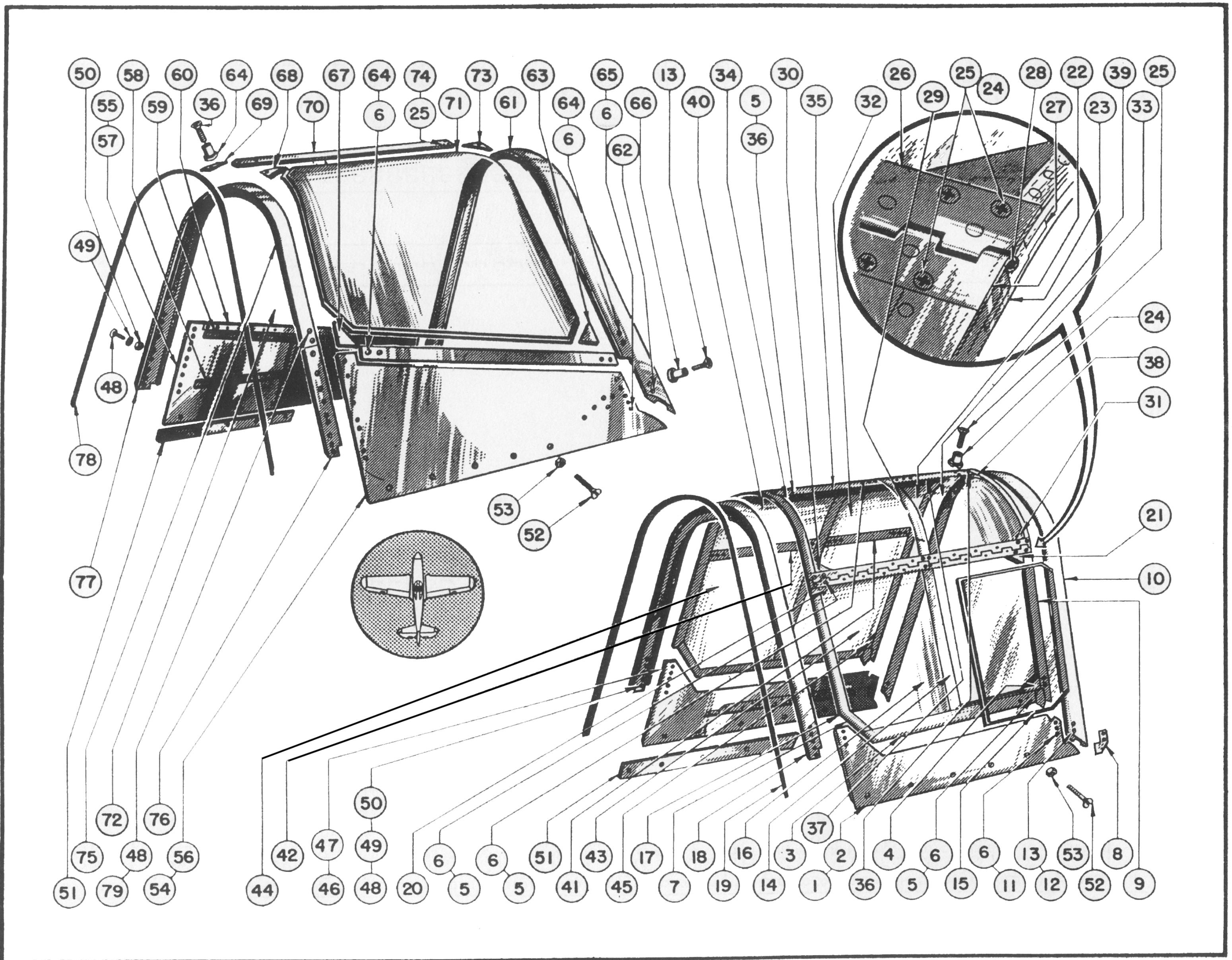
Figure 34 (Sheet 1 of 2 Sheets)—Cabin Assembly
