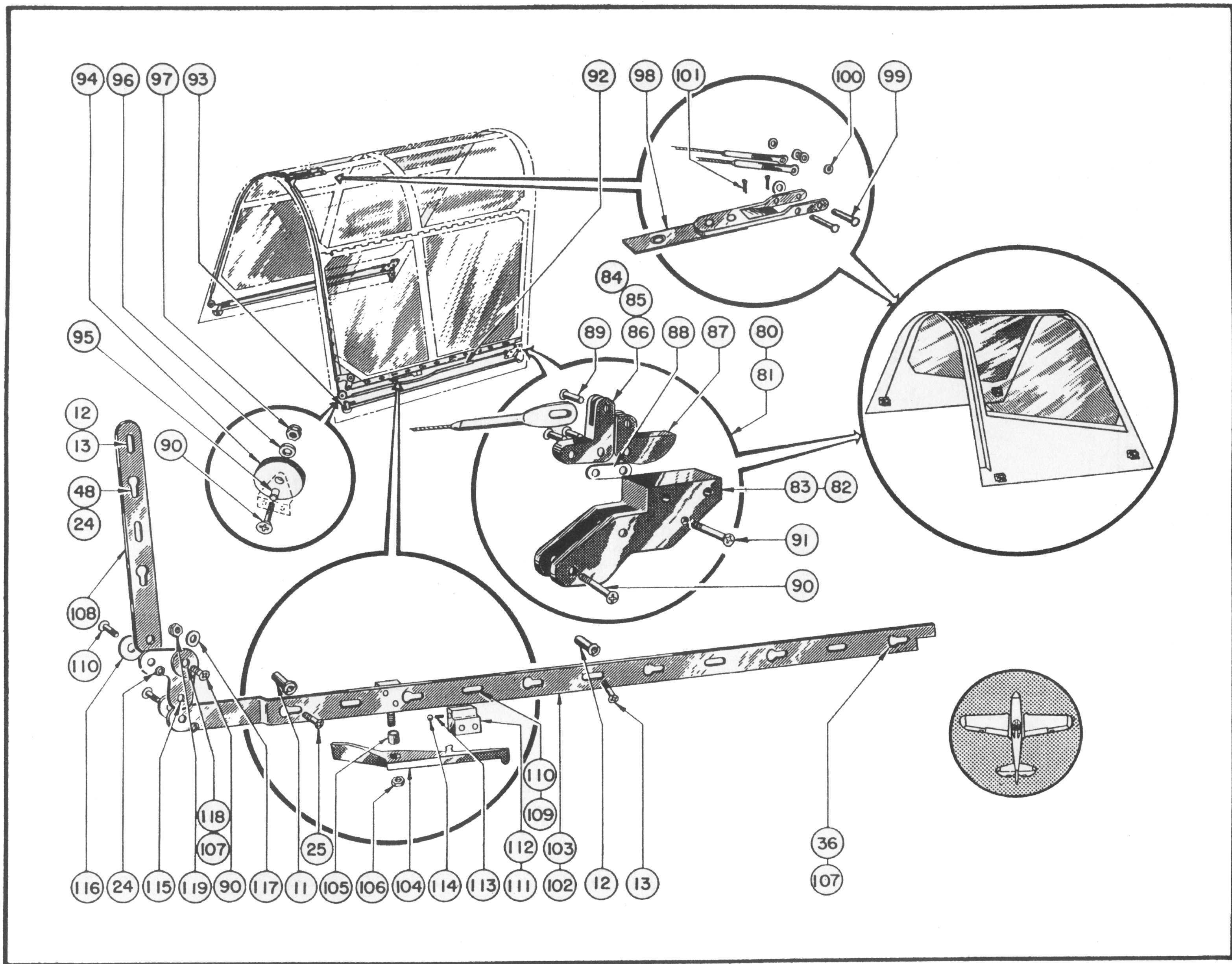
Figure 34 (Sheet 2 of 2 Sheets)—Cabin Assembly
