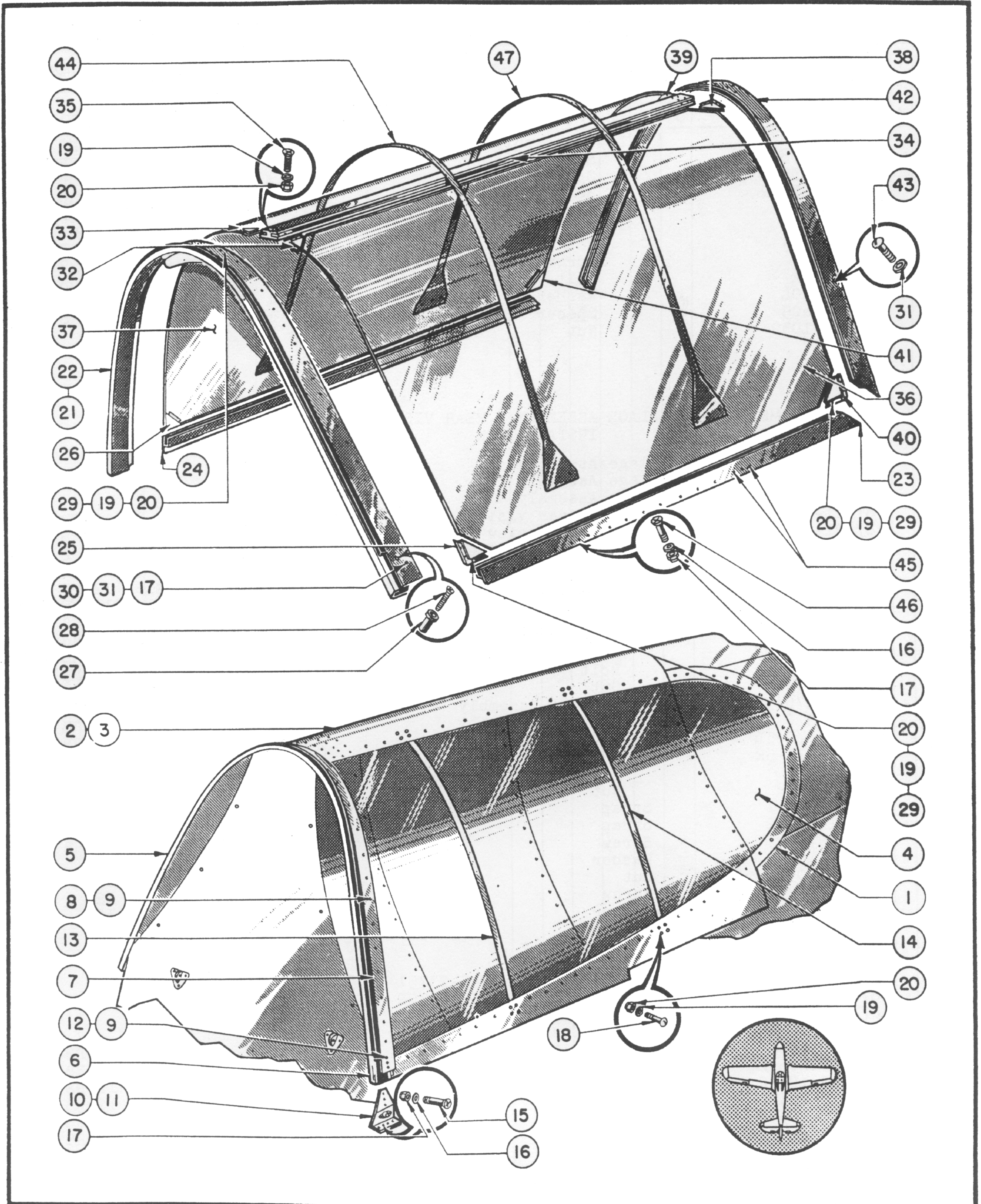
Figure 35—Rear Vision Installation
