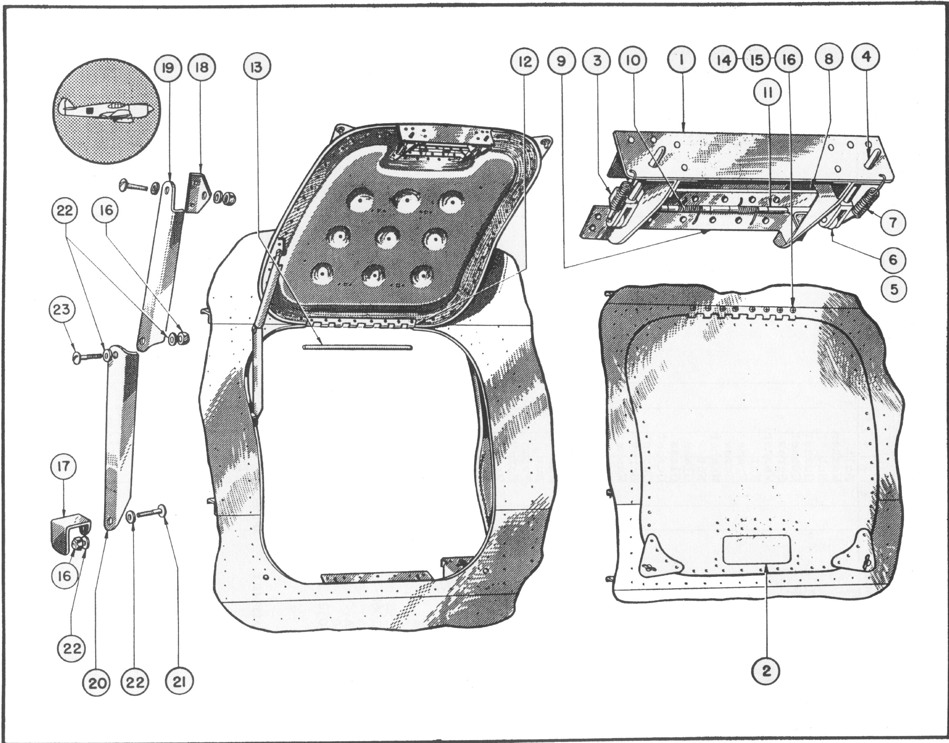
Figure 36—Fuselage Access Door Assembly
