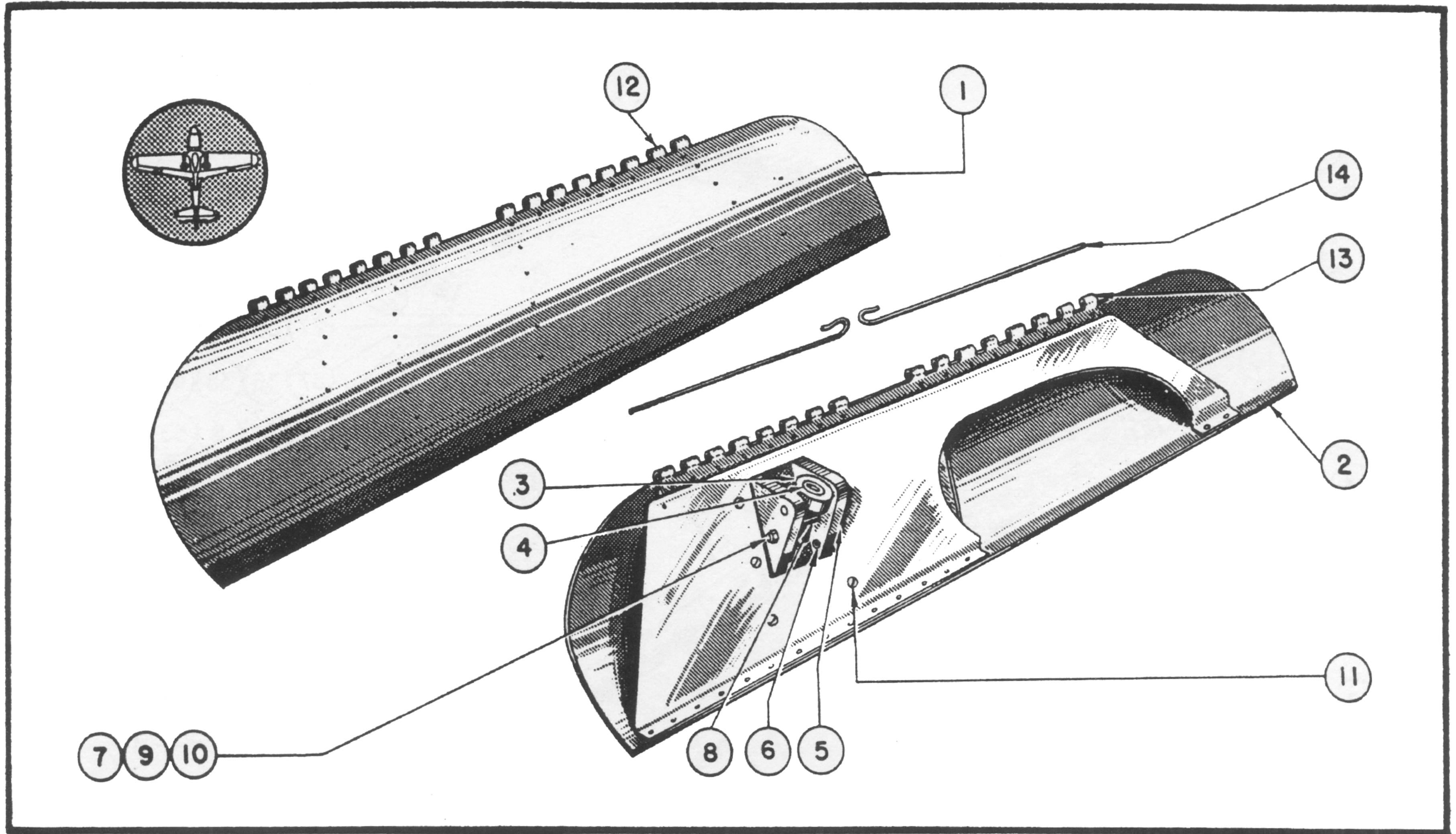
Figure 37—Tail Wheel Door Assembly
