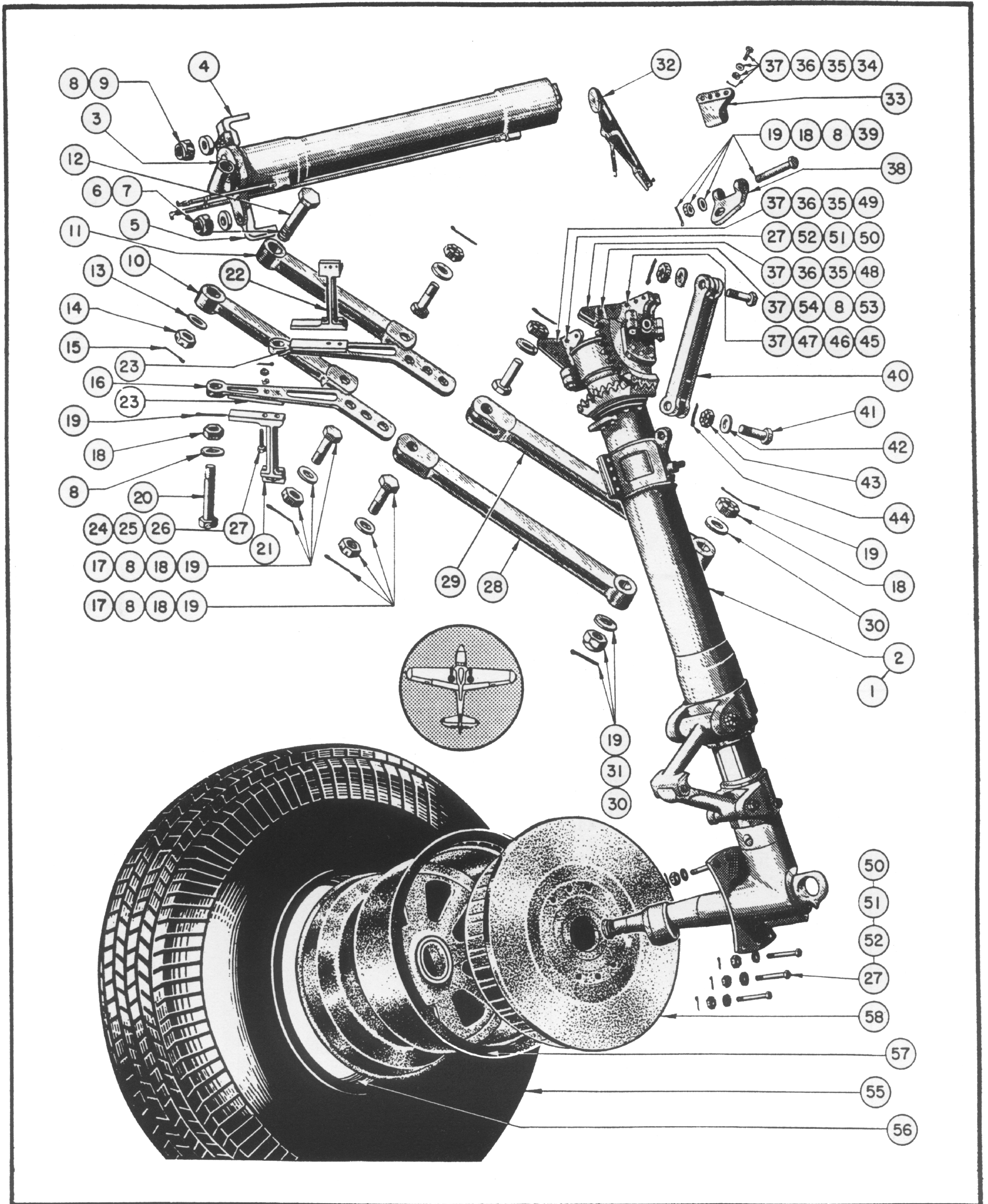
Figure 38—Landing Gear Installation (A-C & W)
