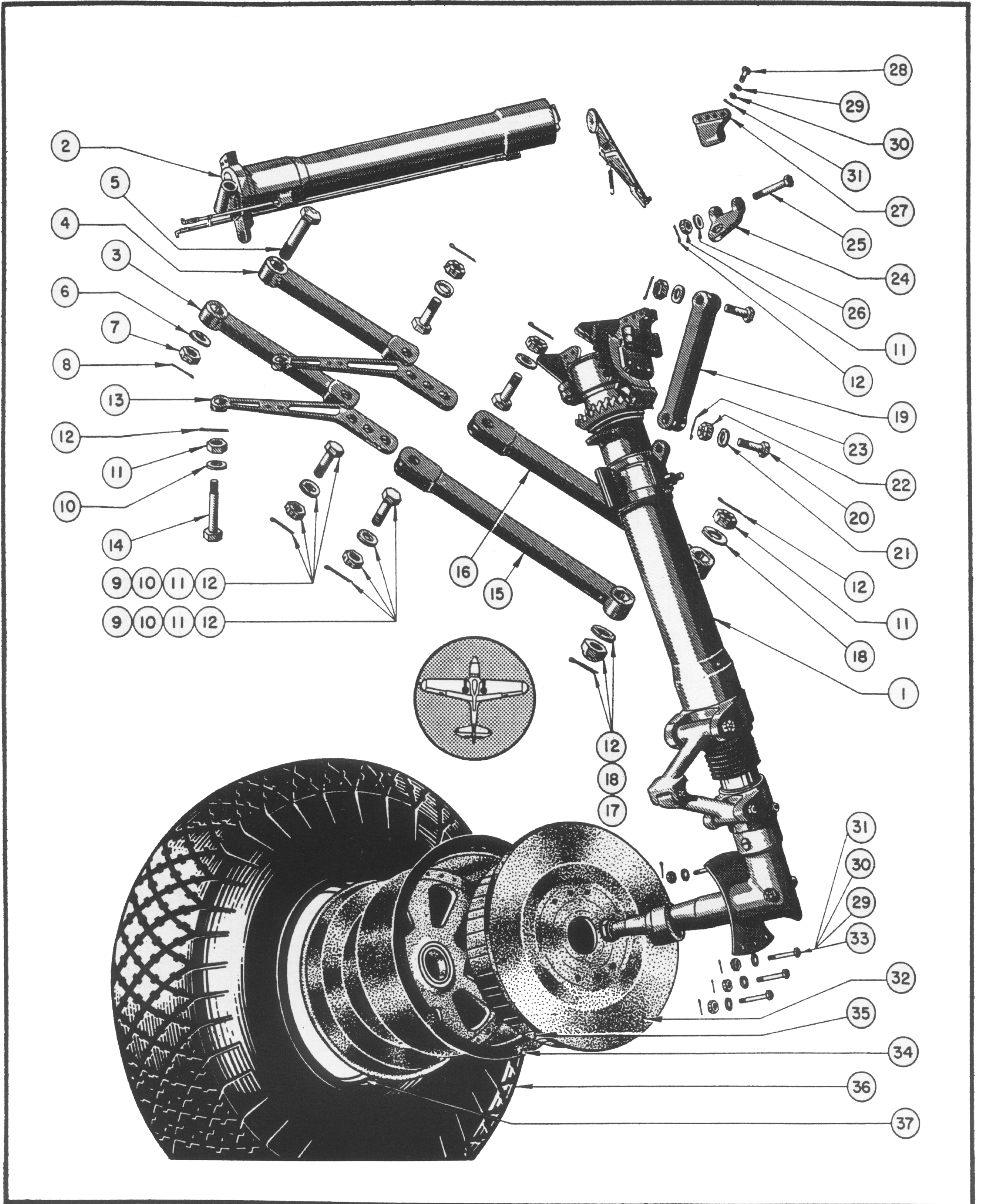
Figure 39—Landing Gear Installation (D-V)
