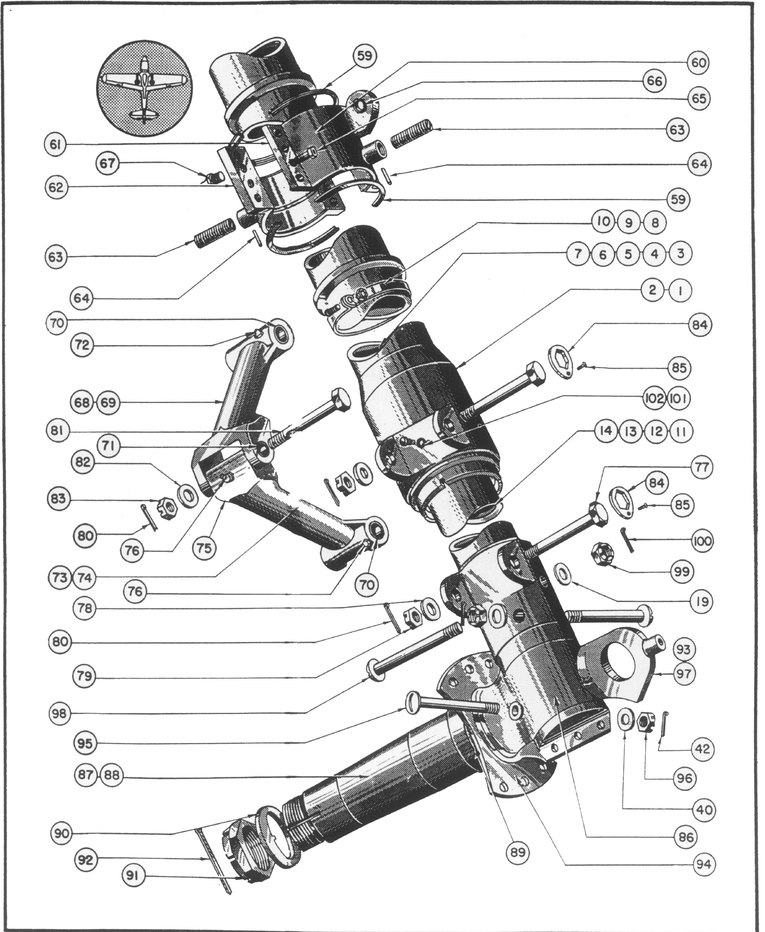
Figure 41 (Sheet 1 of 2 Sheets)—Landing Gear Oleo Strut Assembly
