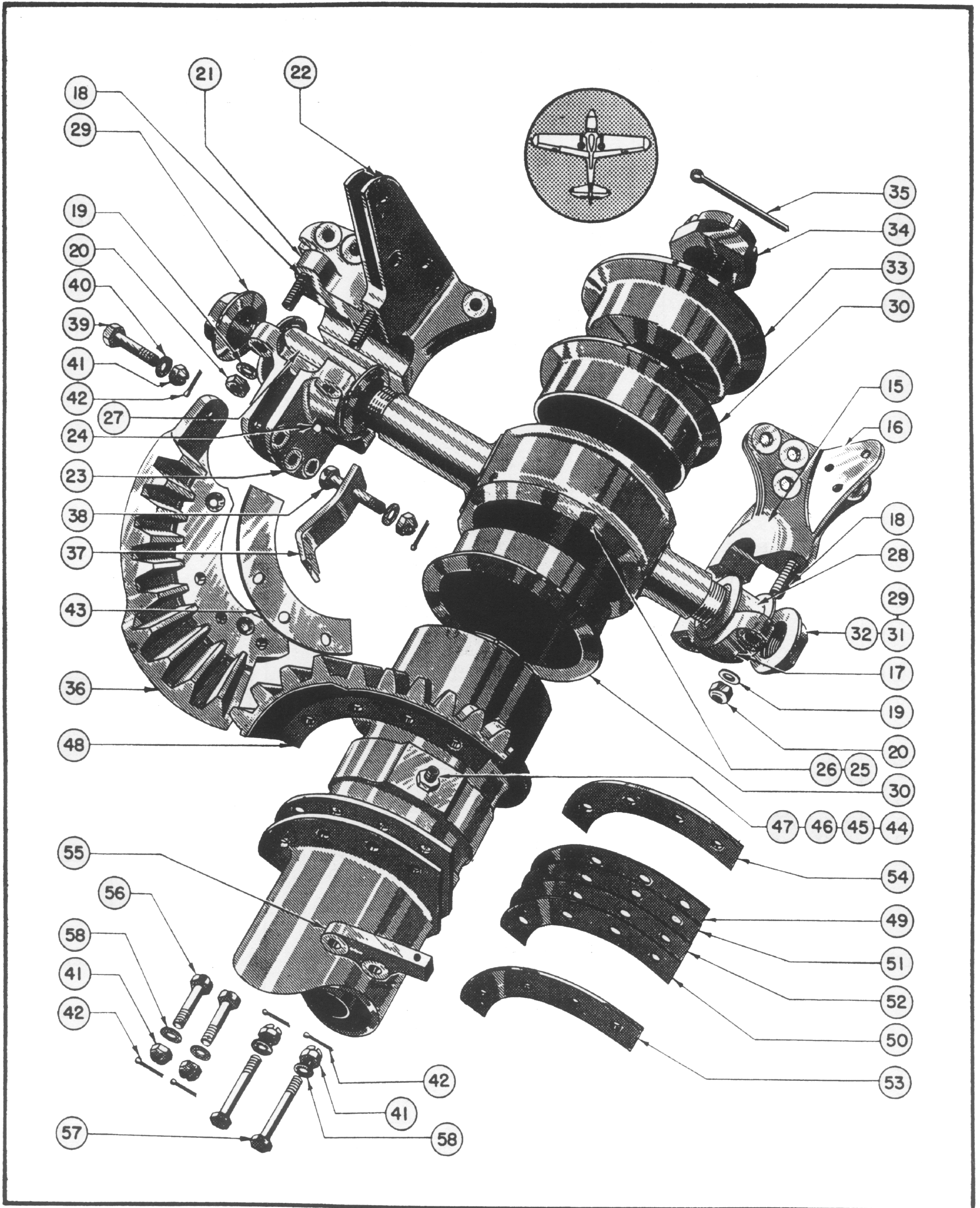
Figure 41 (Sheet 2 of 2 Sheets)—Landing Gear Oleo Strut Assembly
