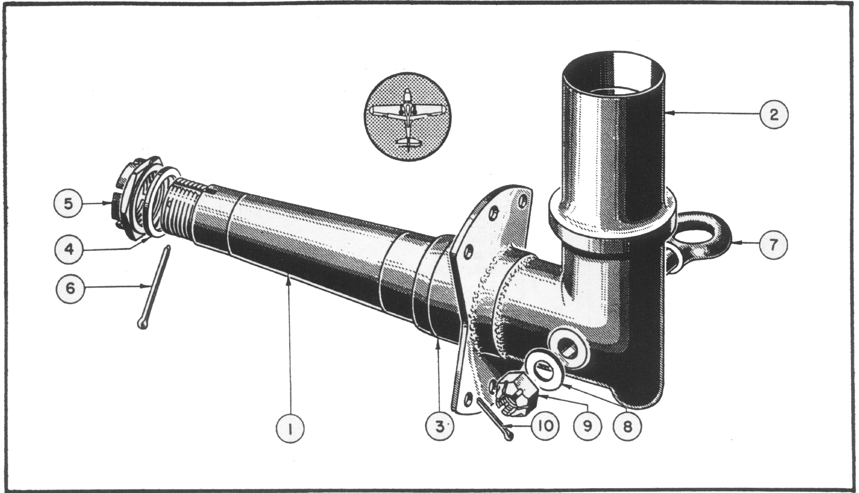
Figure 43—Fitting Assembly
