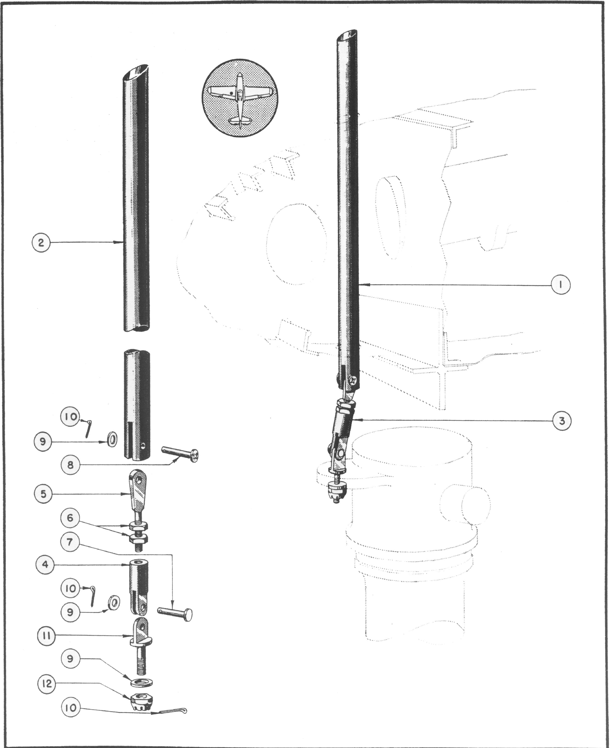
Figure 44—Visual Position Indicator Installation
