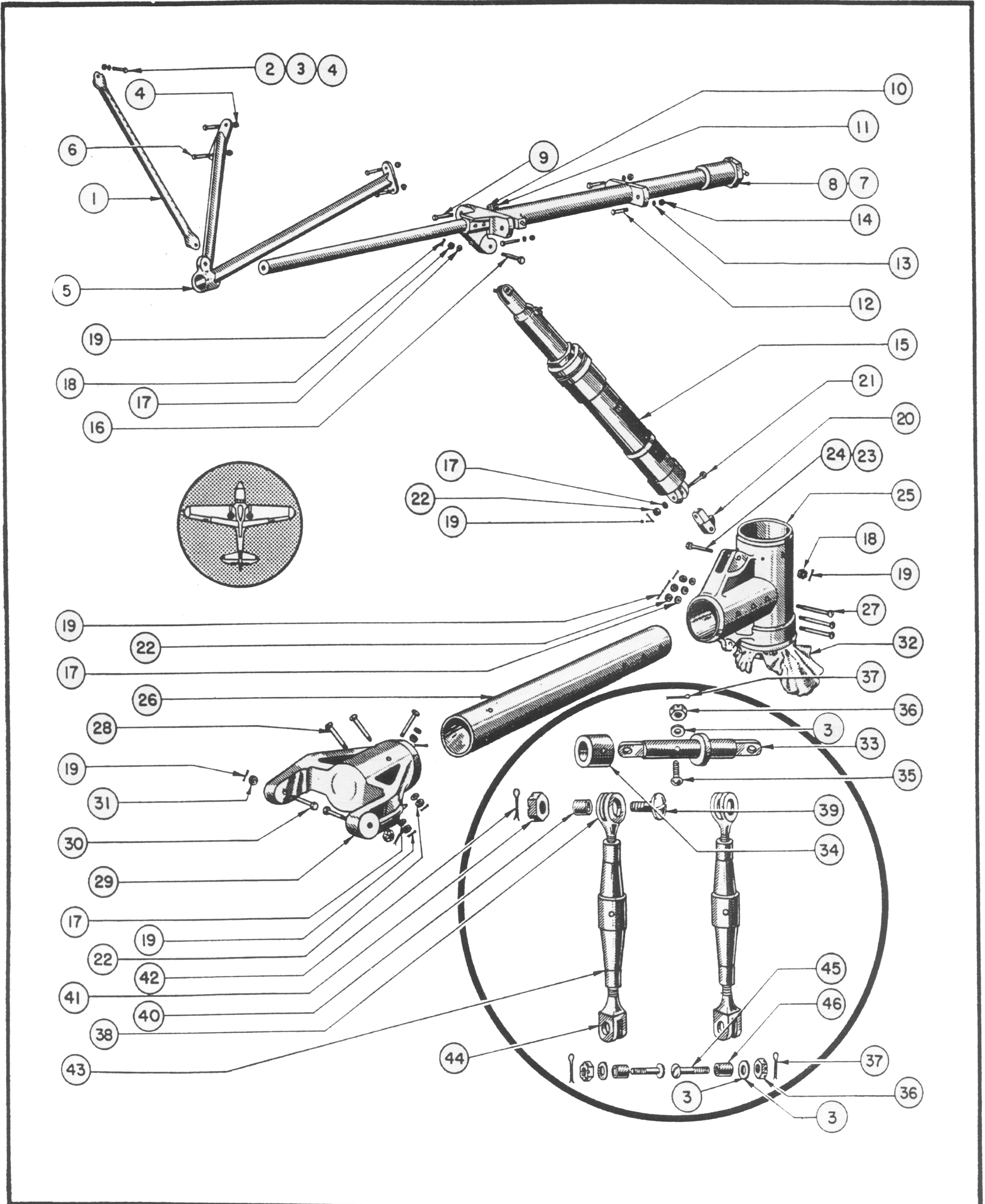
Figure 45 (Sheet 1 of 2 Sheets)—Tail Wheel Installation
