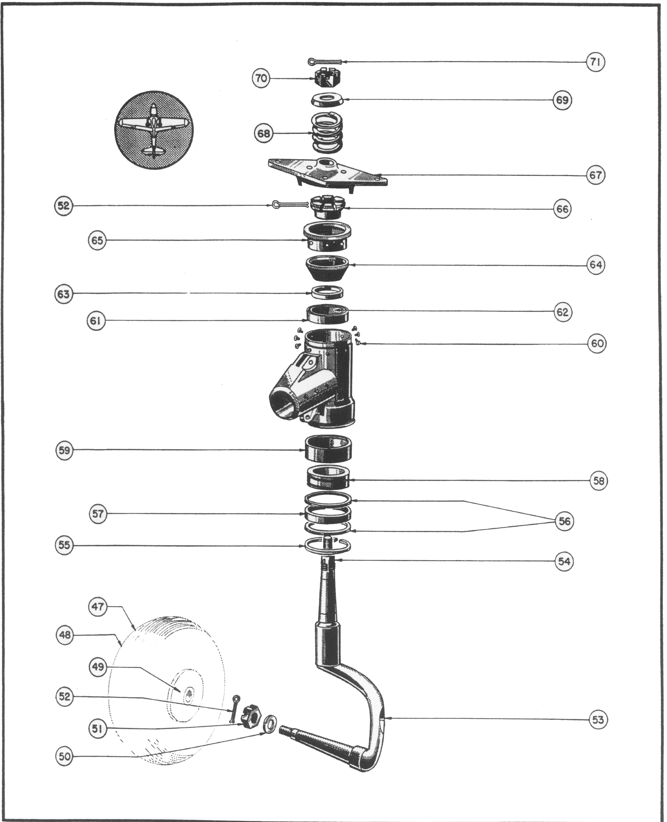
Figure 45 (Sheet 2 of 2 Sheets)—Tail Wheel Installation
