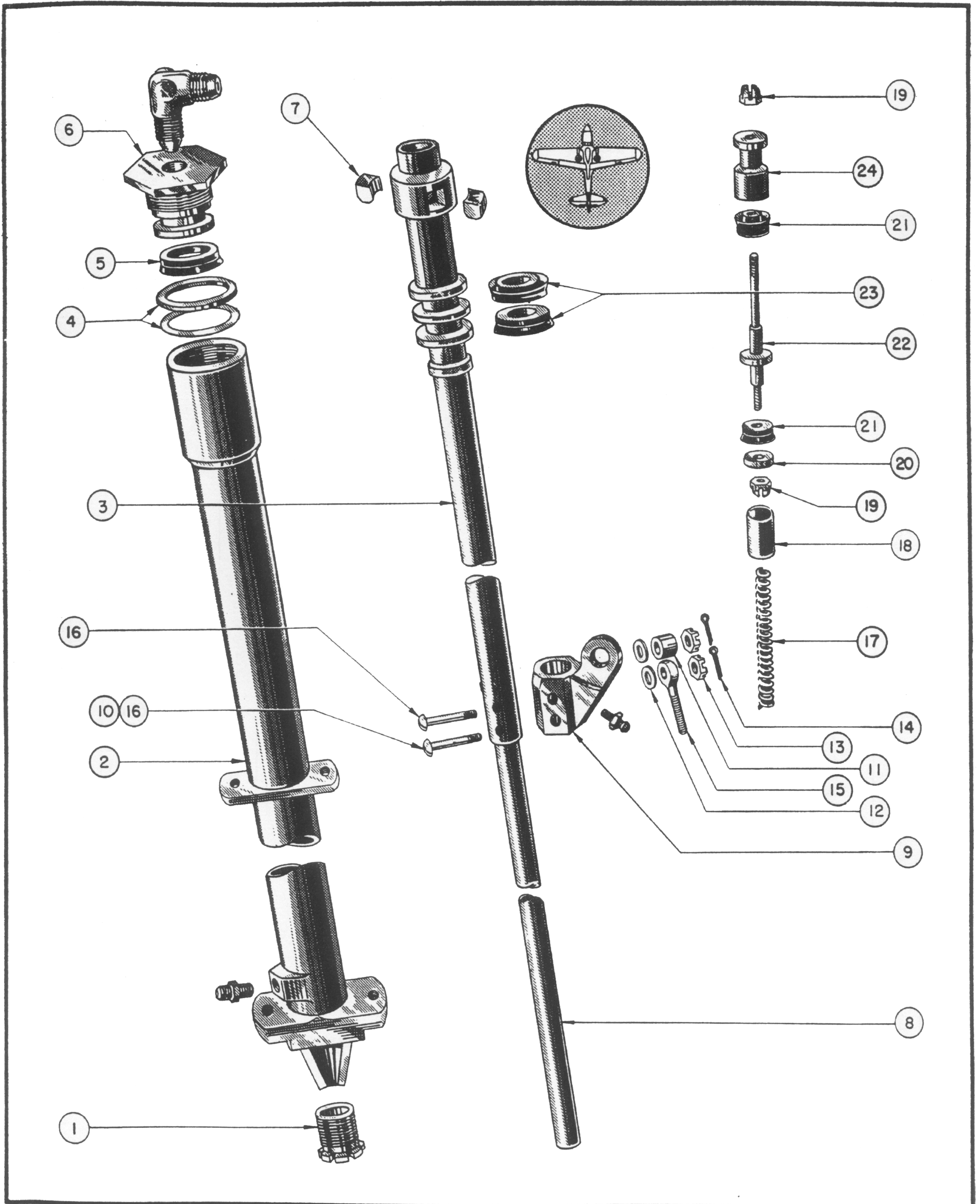
Figure 46—Tail Wheel Retracting Strut
