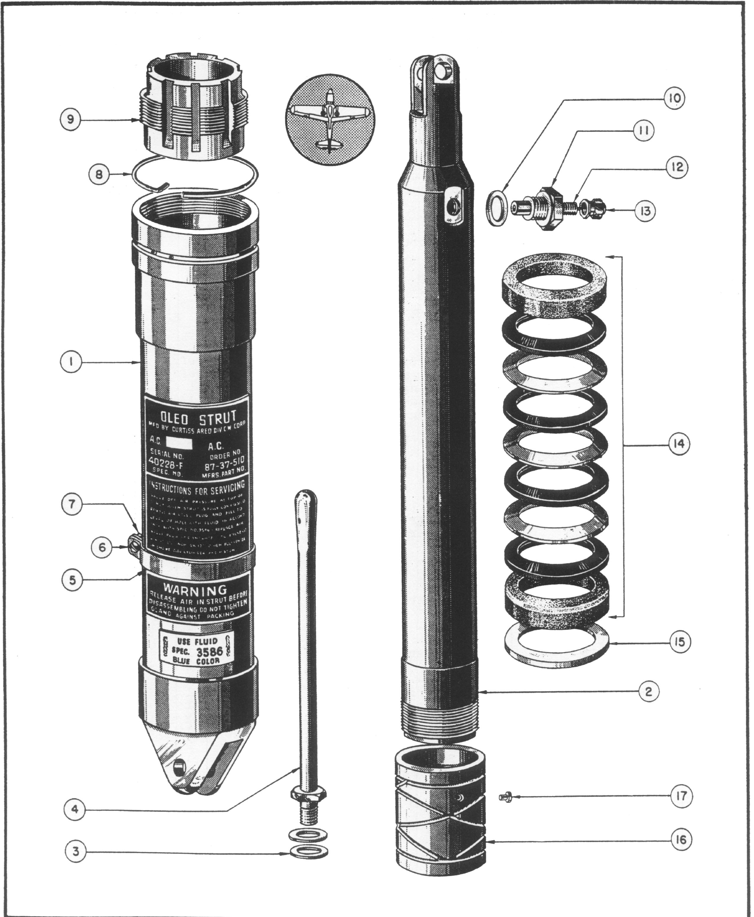
Figure 47—Tail Wheel Oleo Strut Assembly
