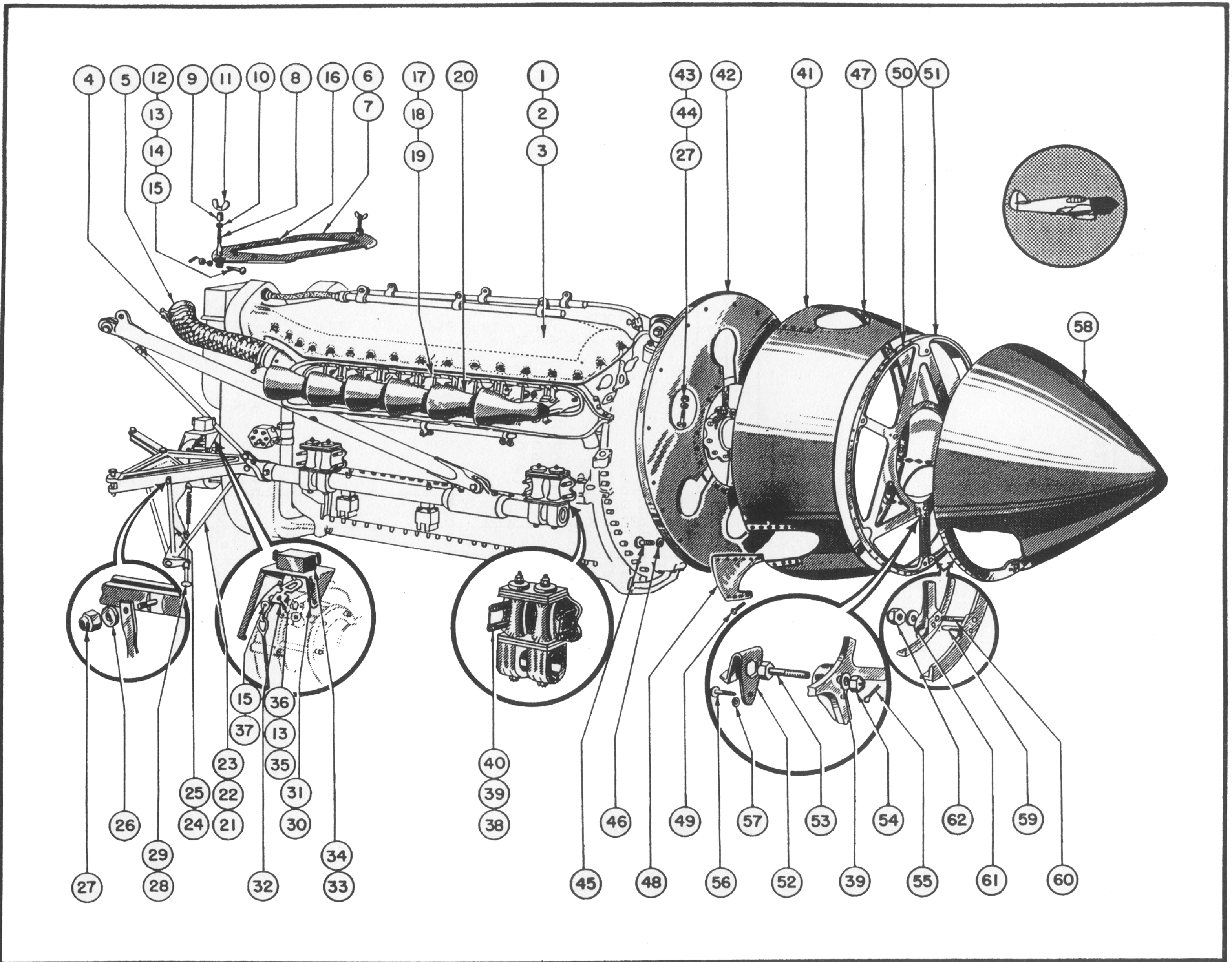
Figure 48—Engine Installation
