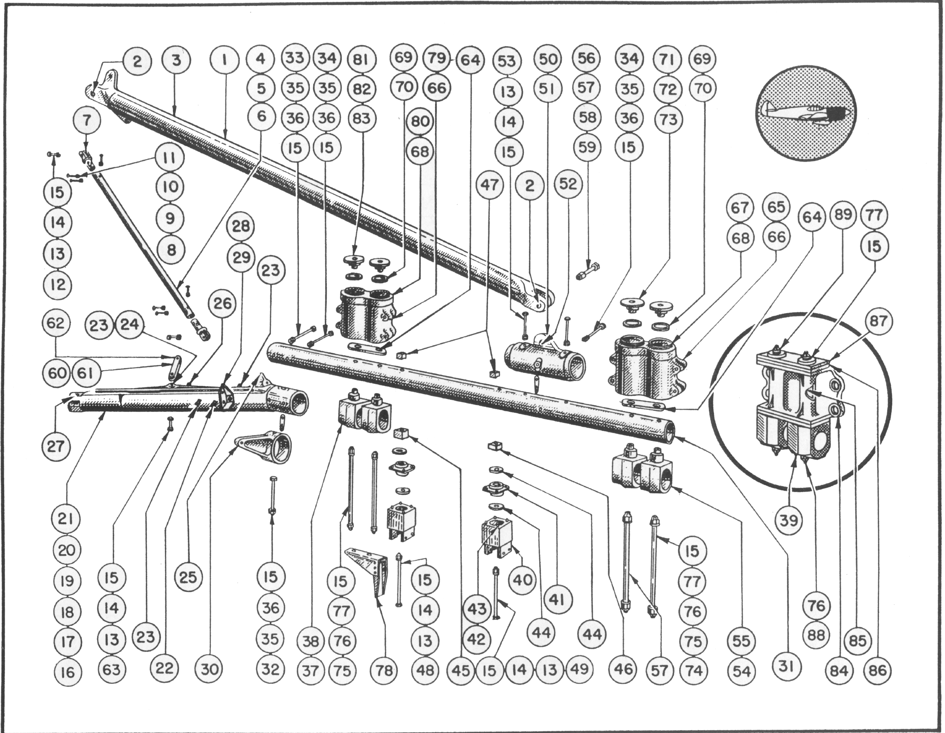
Figure 49—Engine Mount Installation
