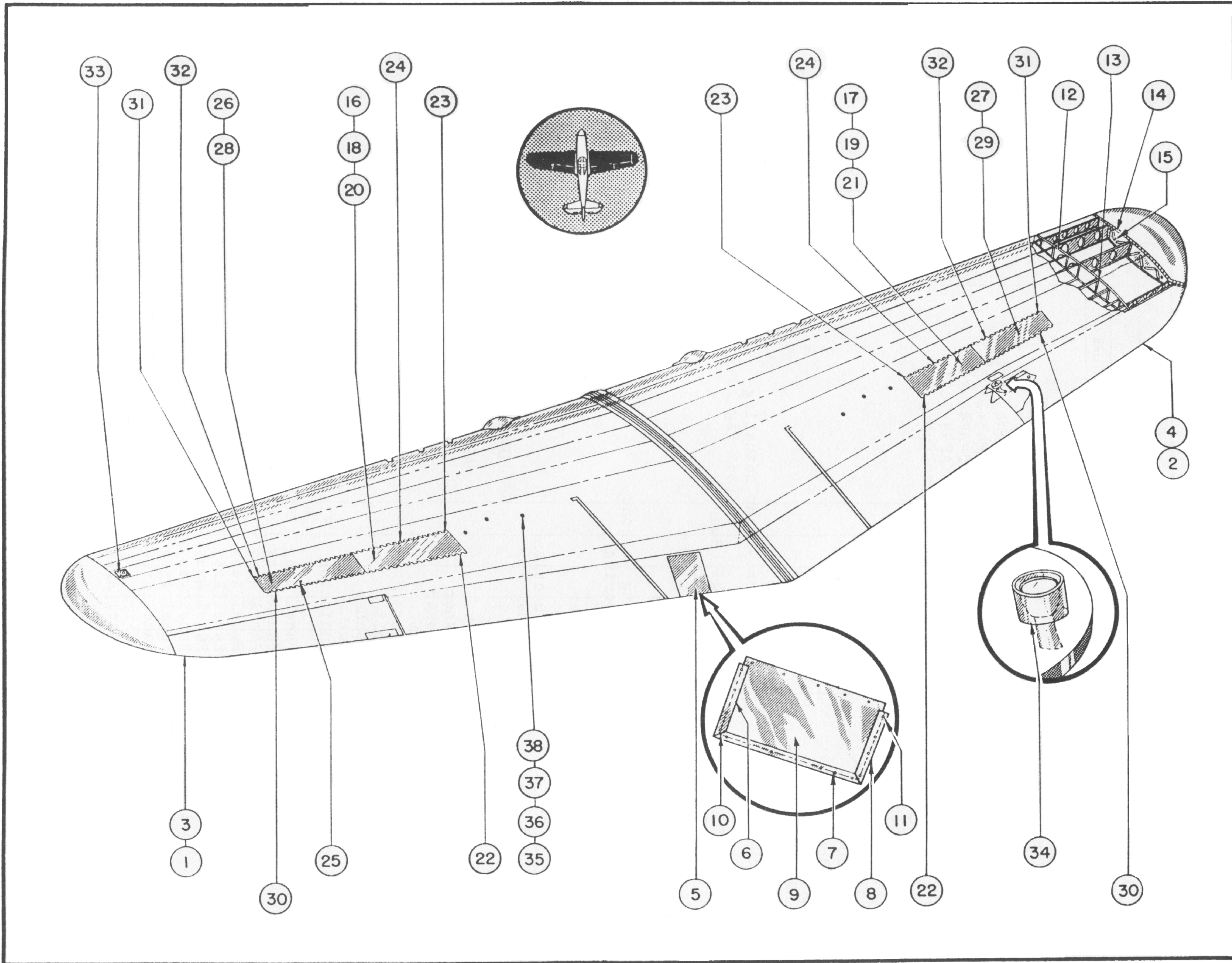
Figure 4 (Sheet 1 of 2 Sheets)—Wing Panel Assembly
