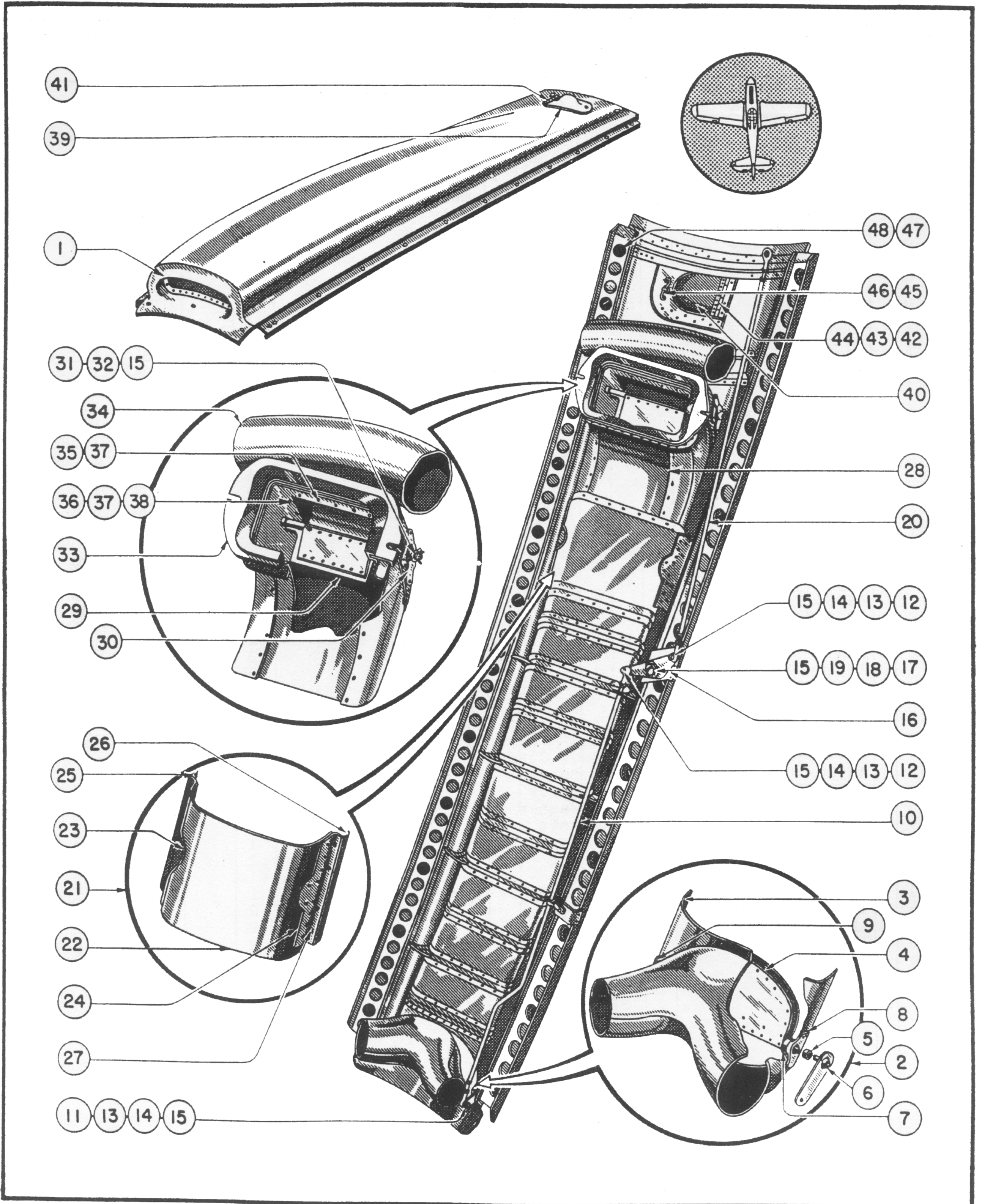
Figure 52—Engine Top Center Cowling (V-W)
