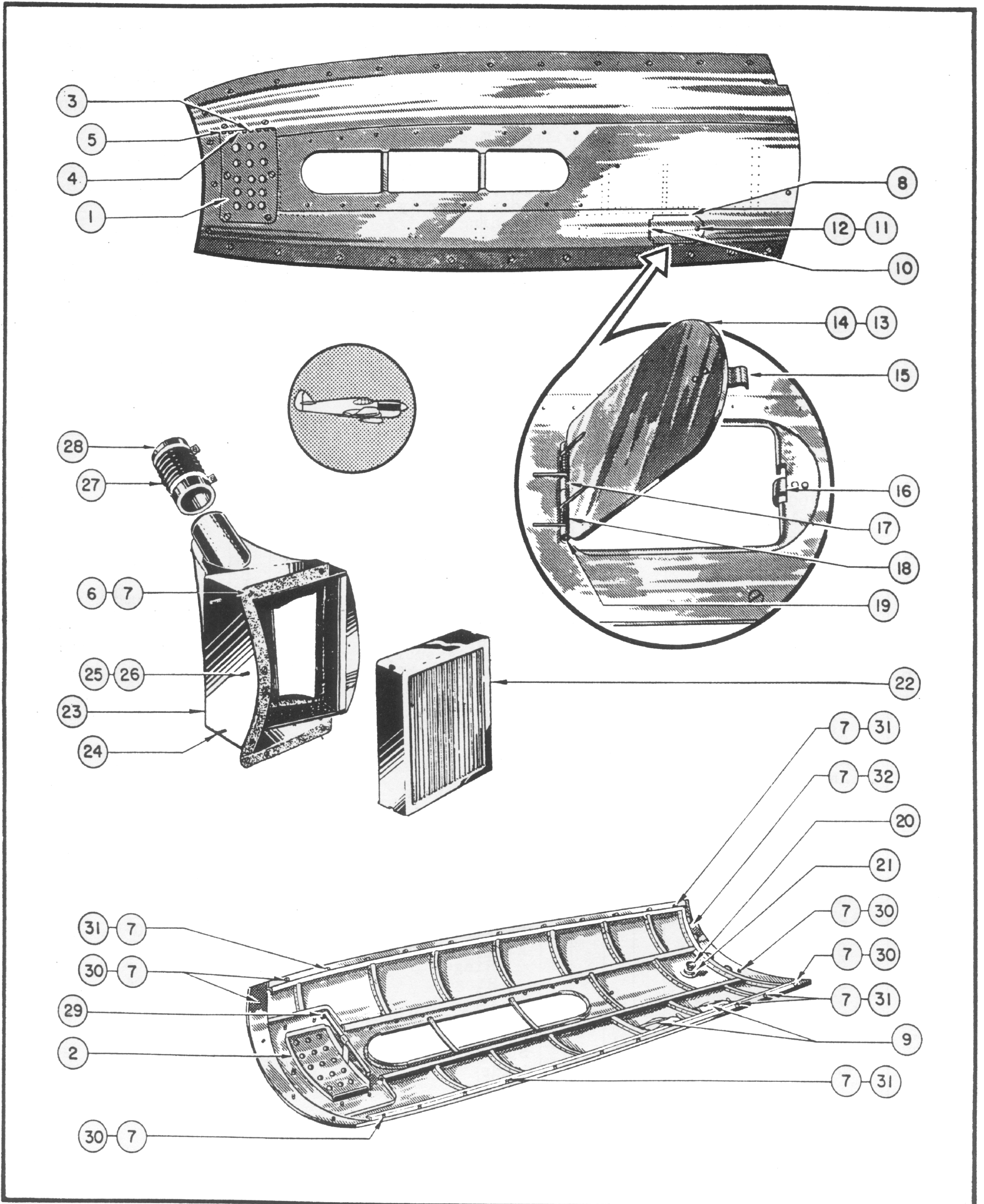
Figure 53—Side Cowling and Air Filter
