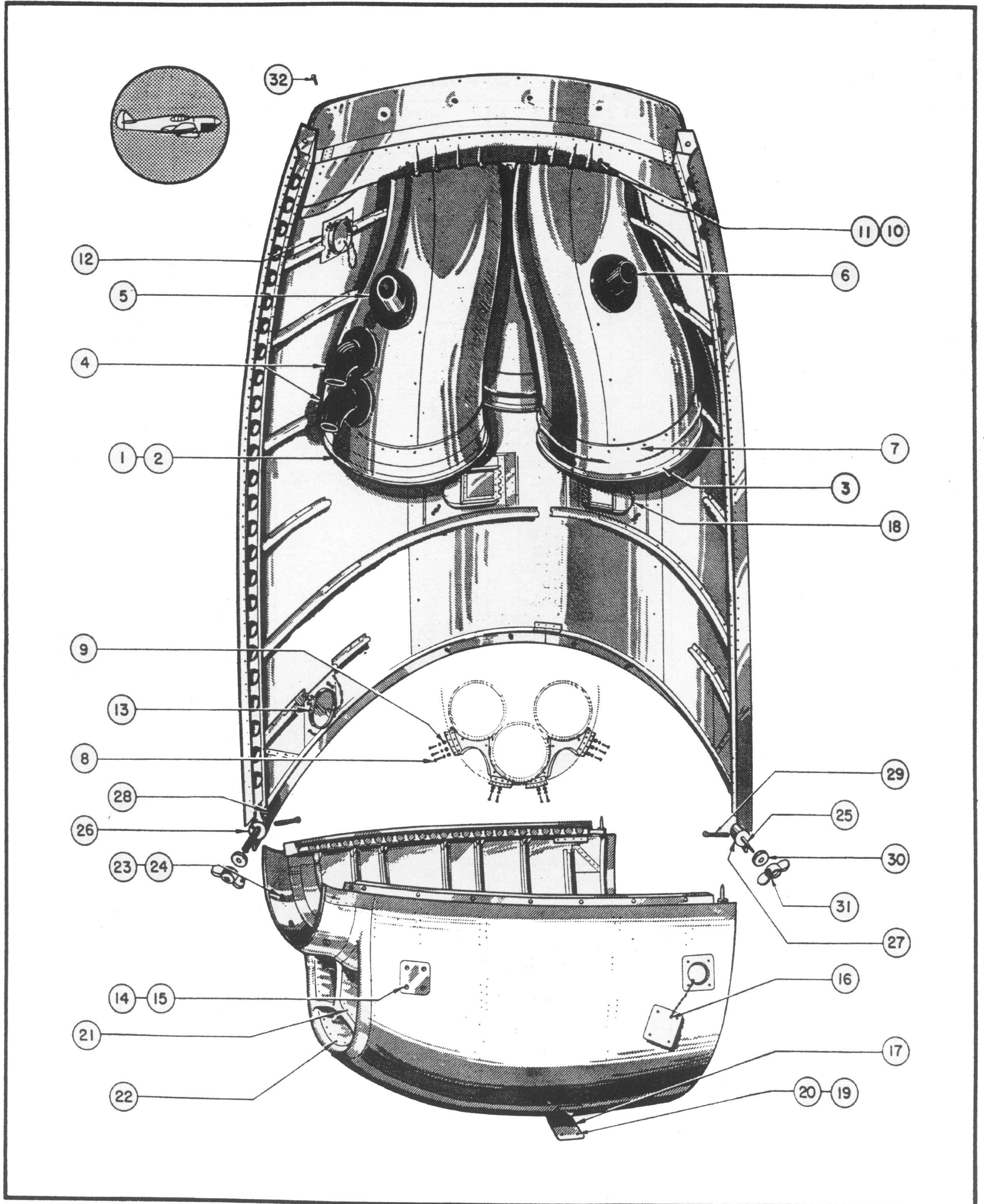
Figure 54—Bottom Forward Cowling Assembly
