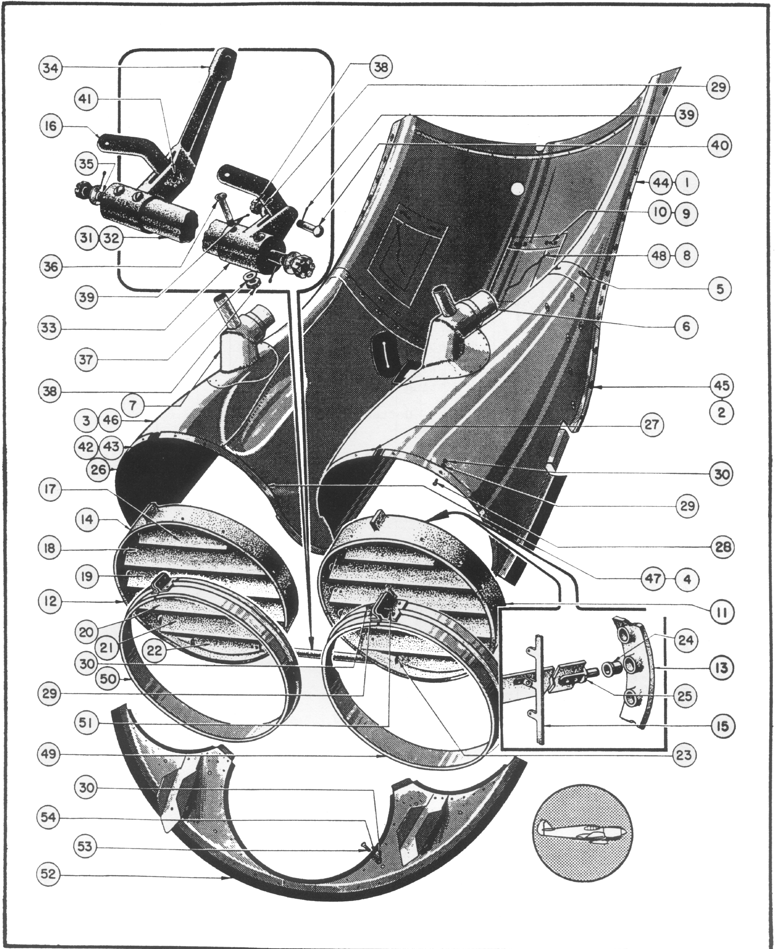
Figure 55—Exit Duct Assembly RESTRICTED
