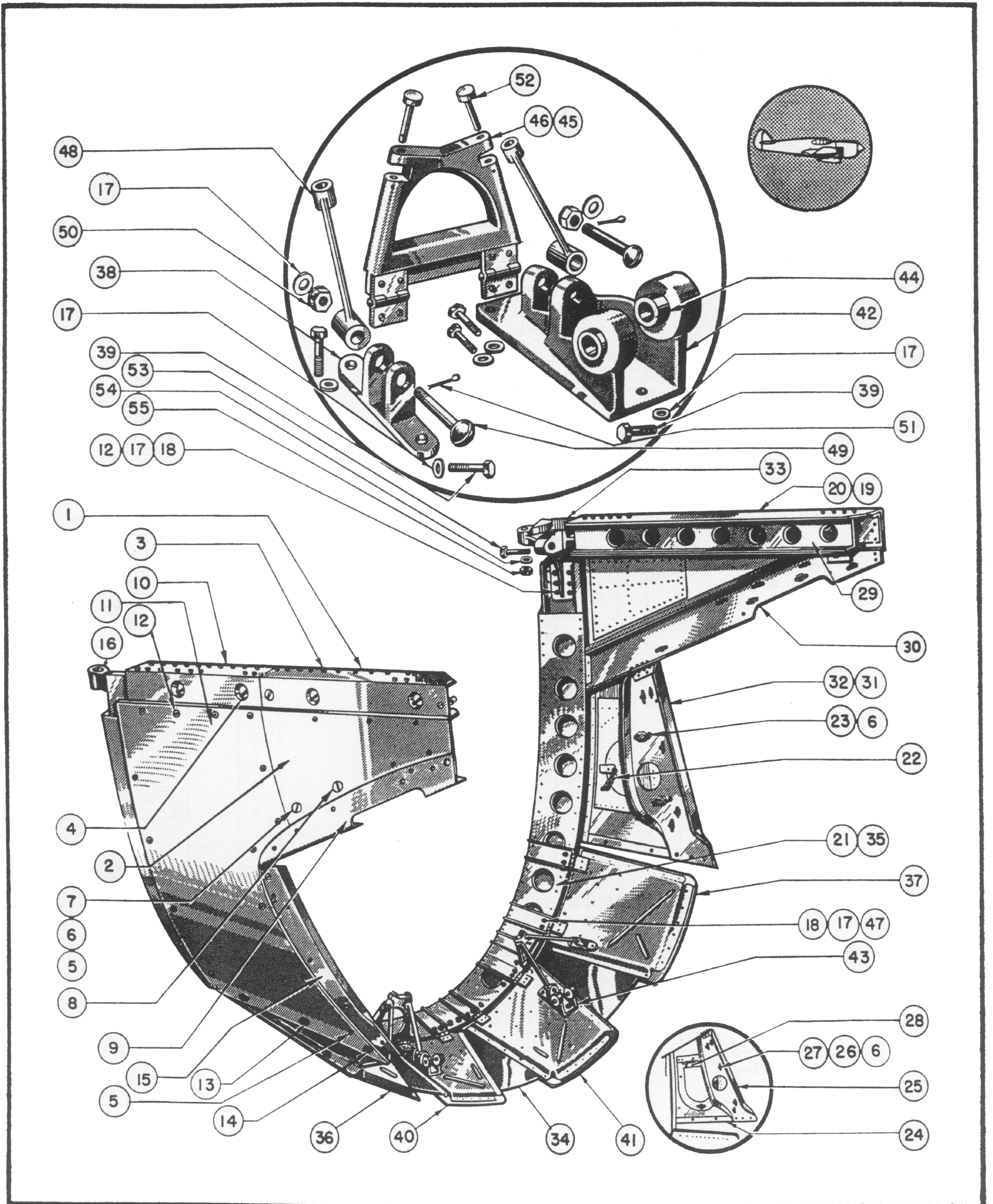
Figure 56—Rear Cowling and Cowl Flaps
