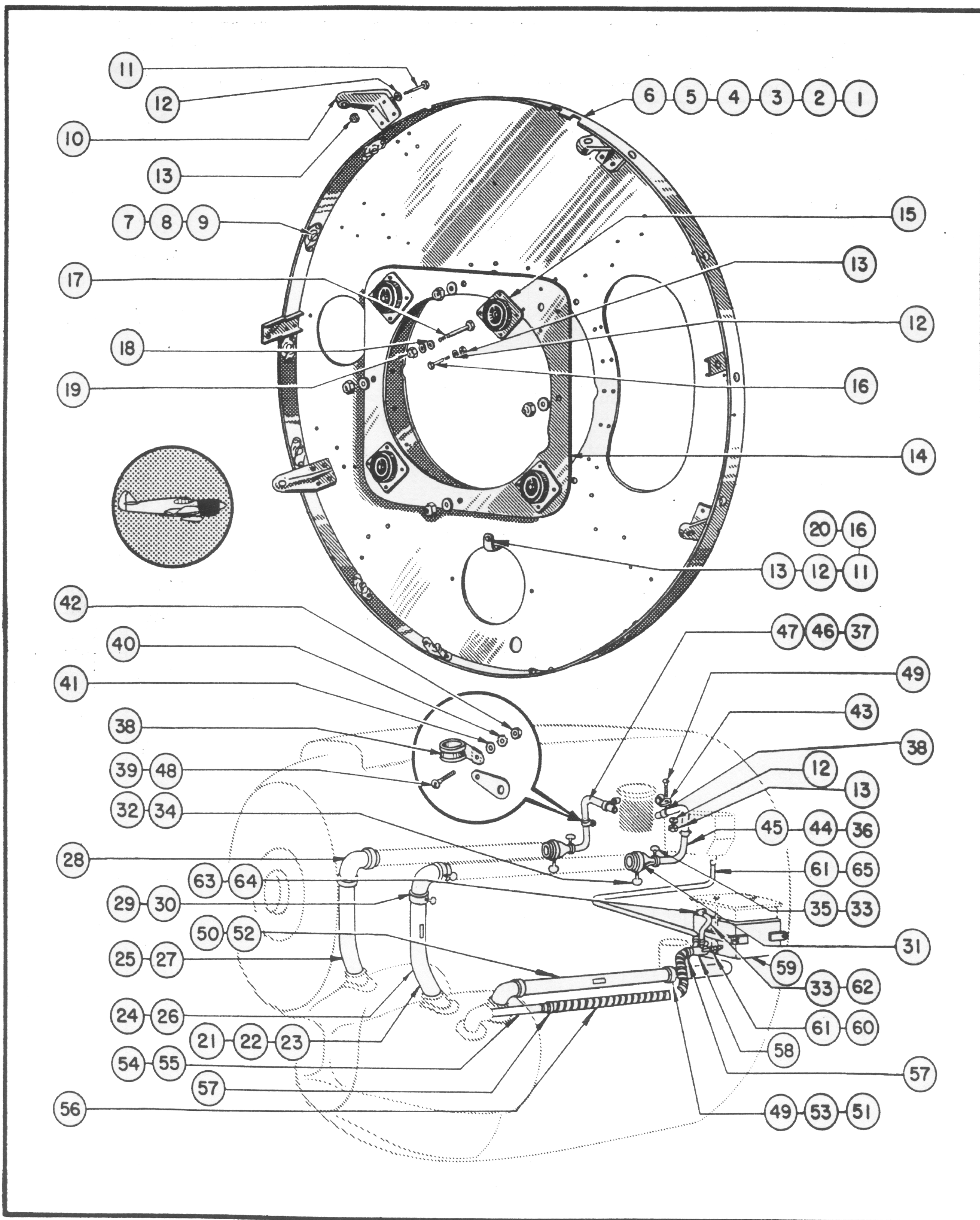
Figure 57—Engine Cowling Bulkhead & Engine Accessories Cooling Tubes Installation
