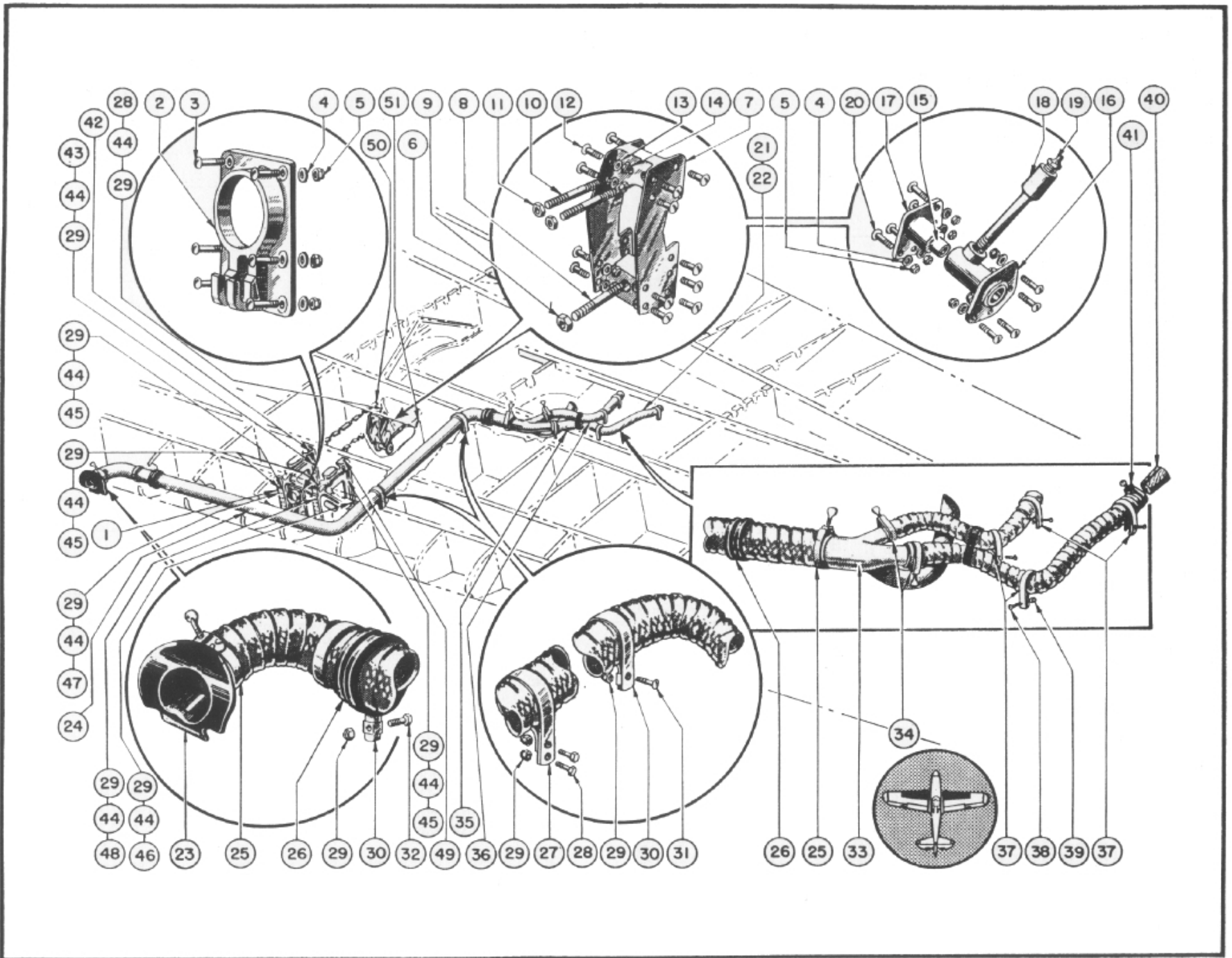
Figure 6—Landing Gear Support and Gun Heater Installation
