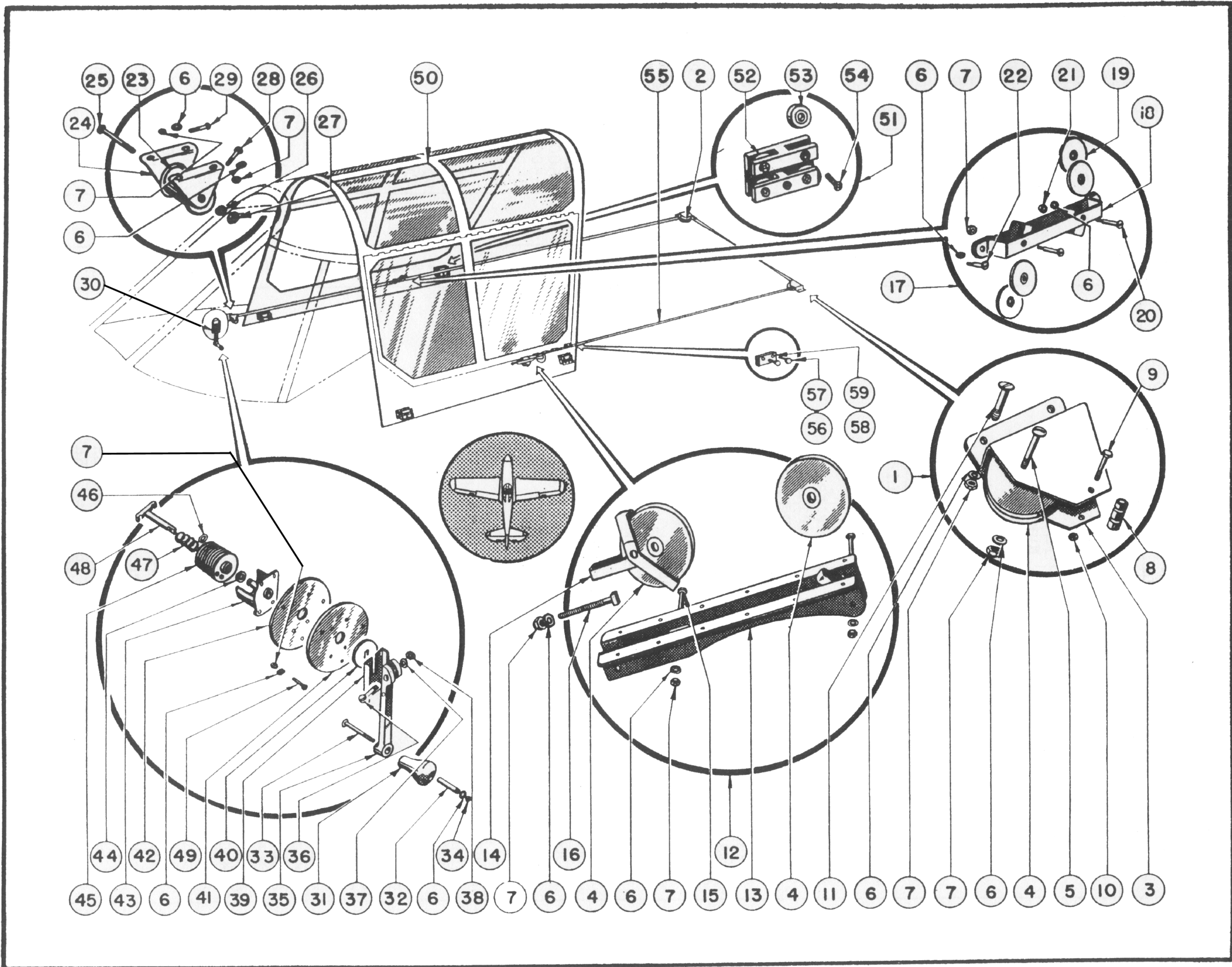
Figure 60—Cabin Controls Installation (A-C)
