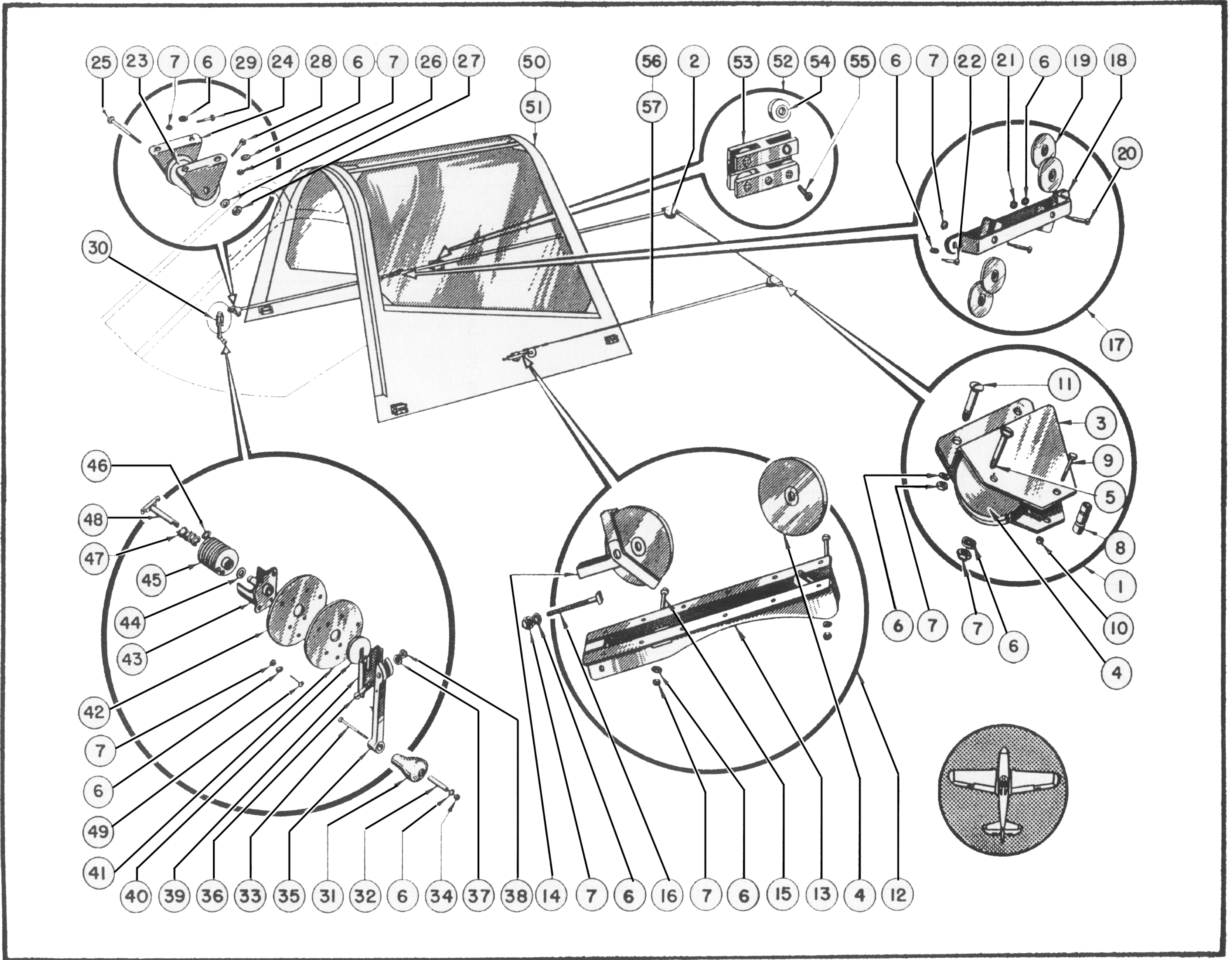
Figure 61—Cabin Controls Installation (D-W)
