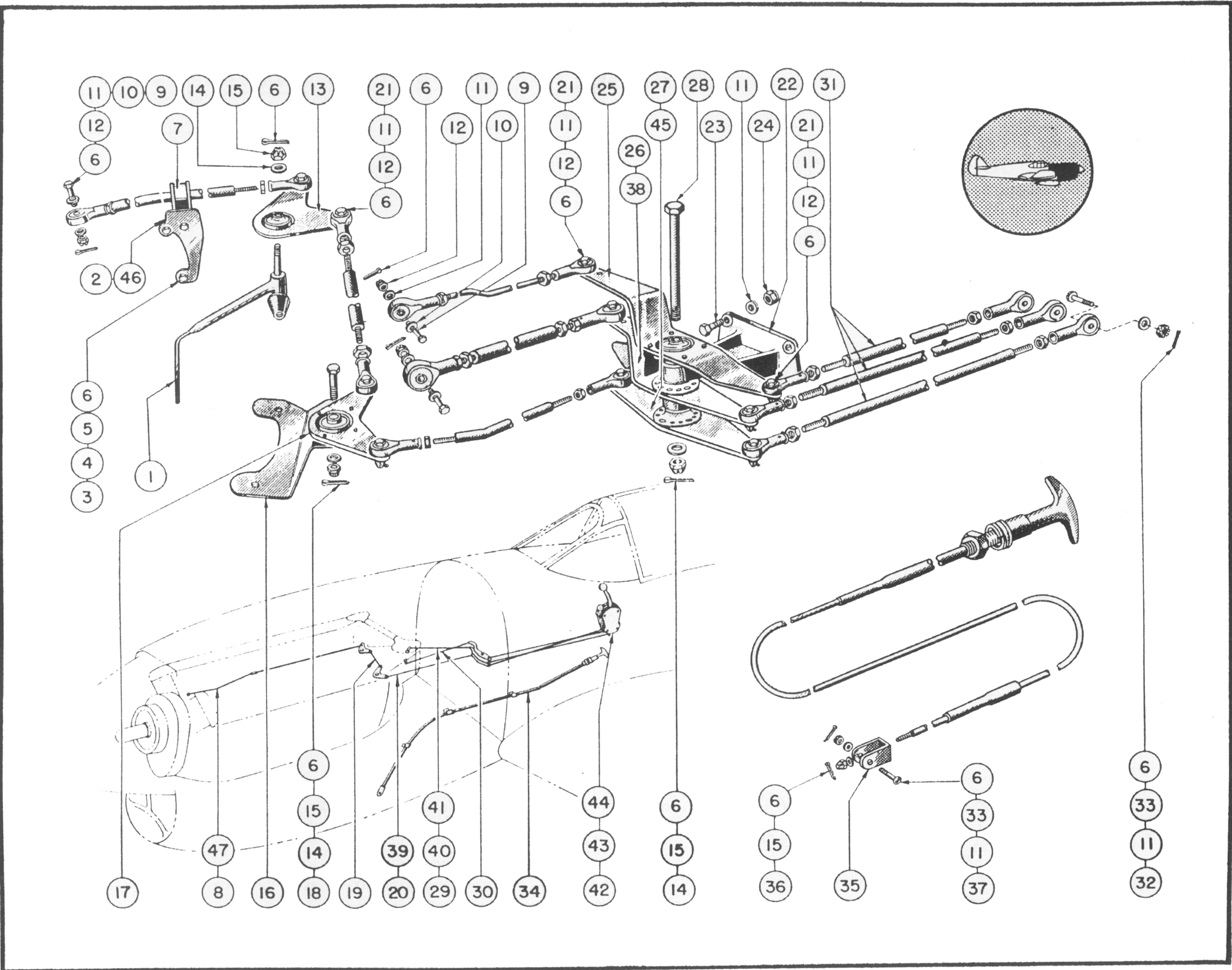
Figure 62—Engine Controls Installation
