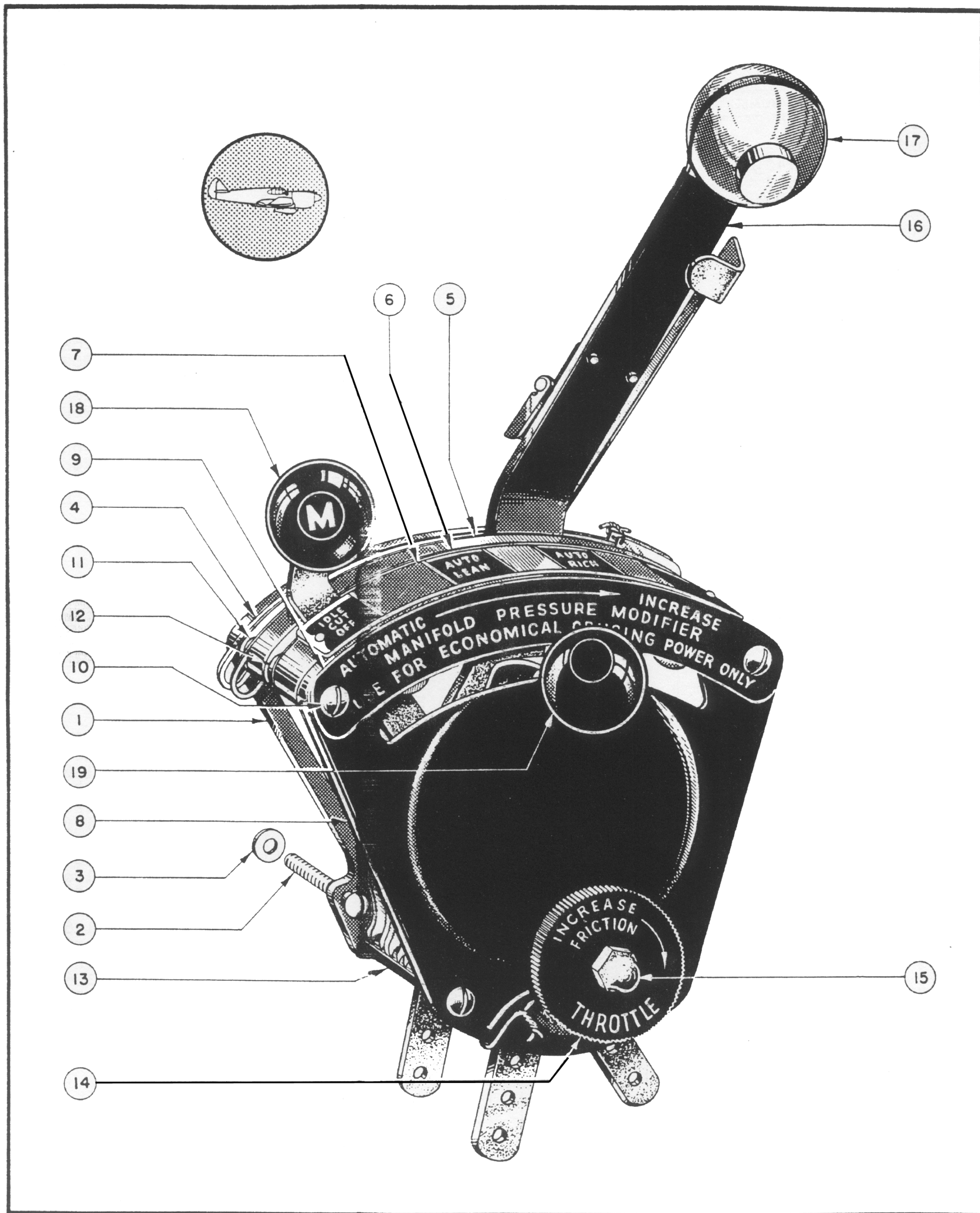
Figure 63—Special Engine Controls Assembly
