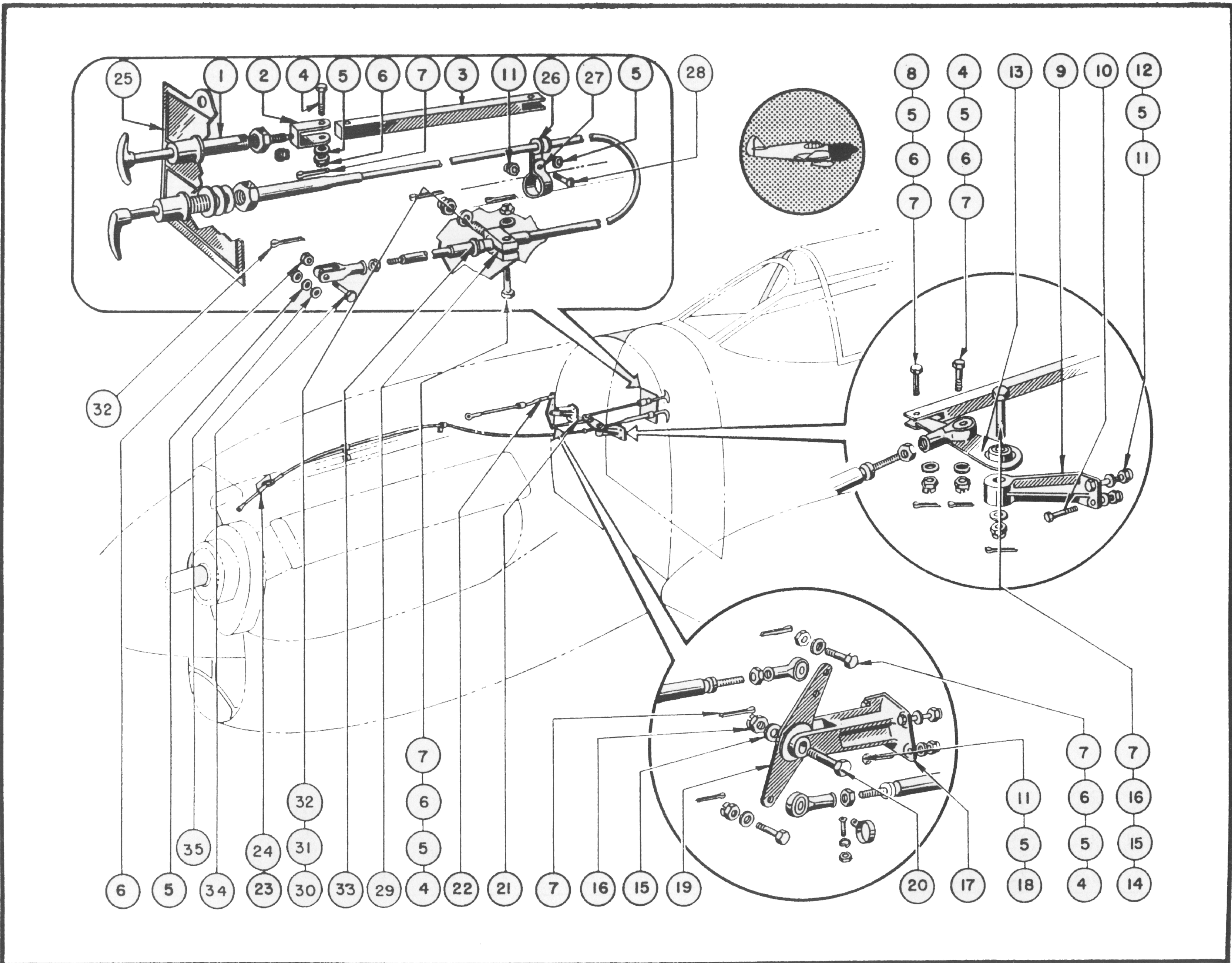
Figure 64—Carburetor Air Heat Controls Installation (A-B)
