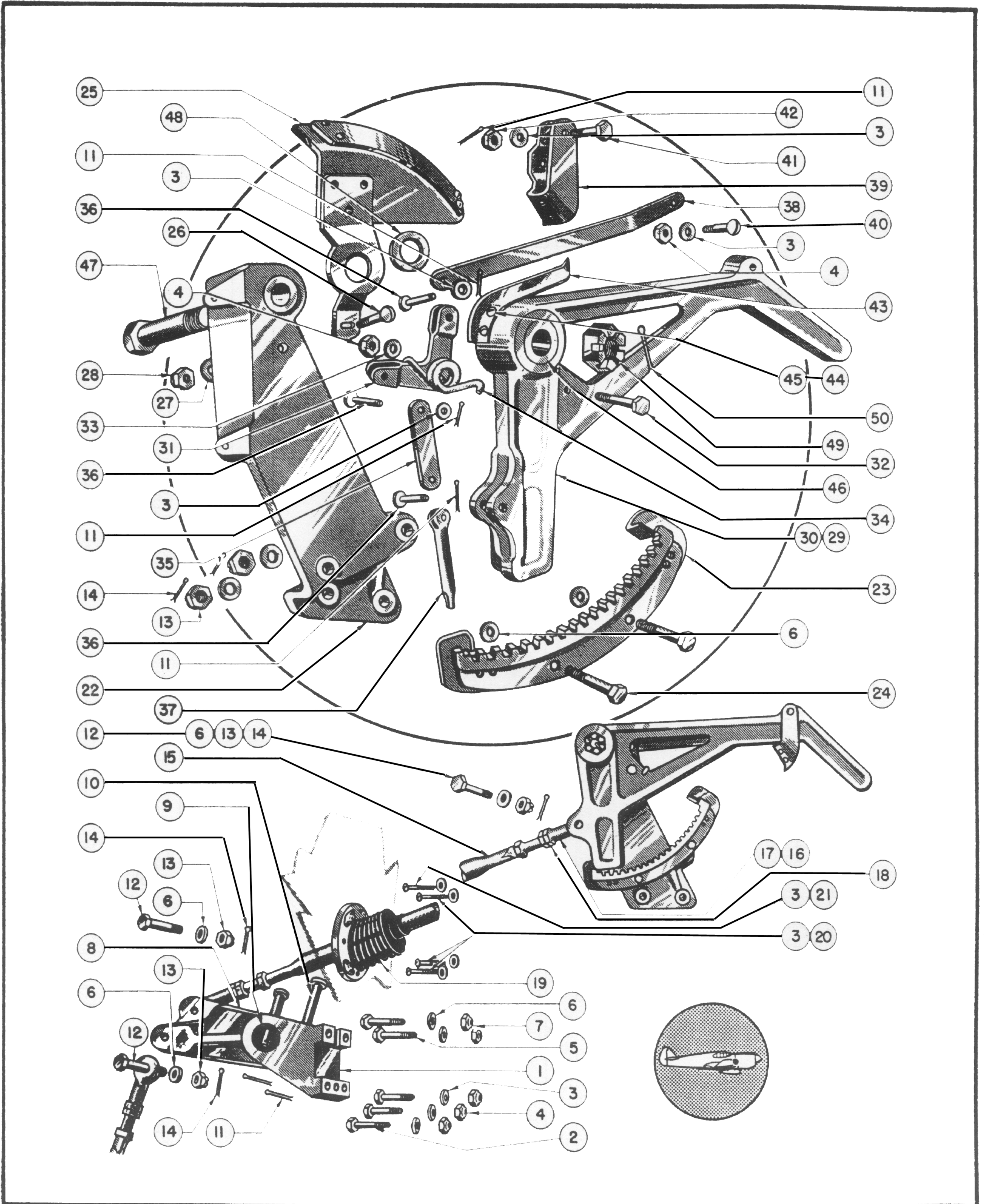
Figure 67—Cowl Flap Controls Installation
