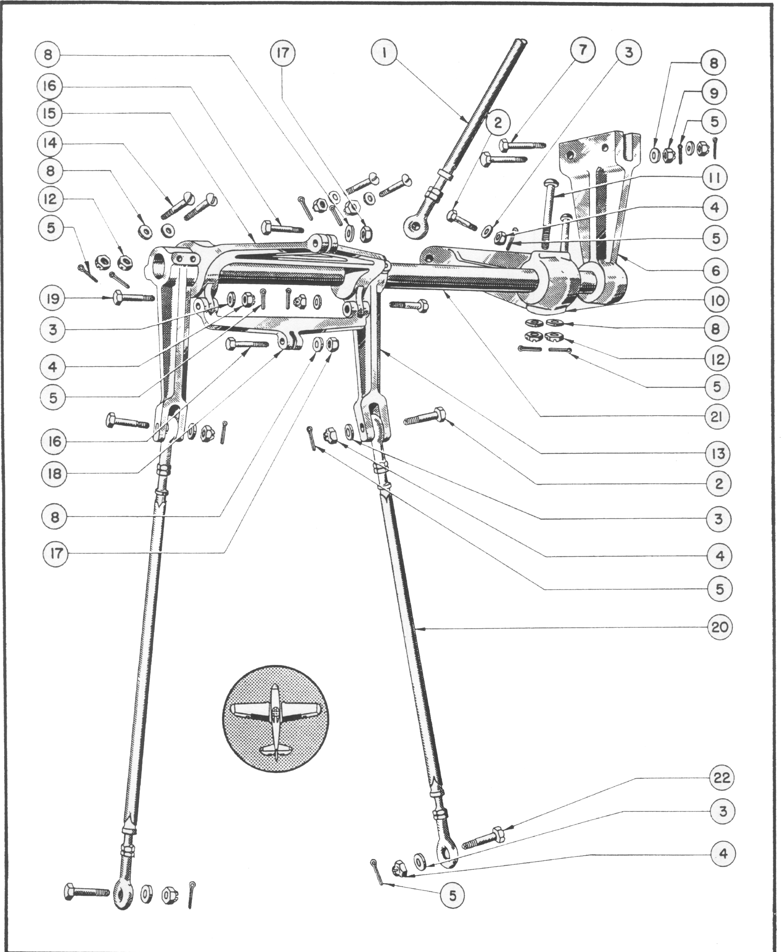
Figure 68—Cowl Flap Controls Installation
