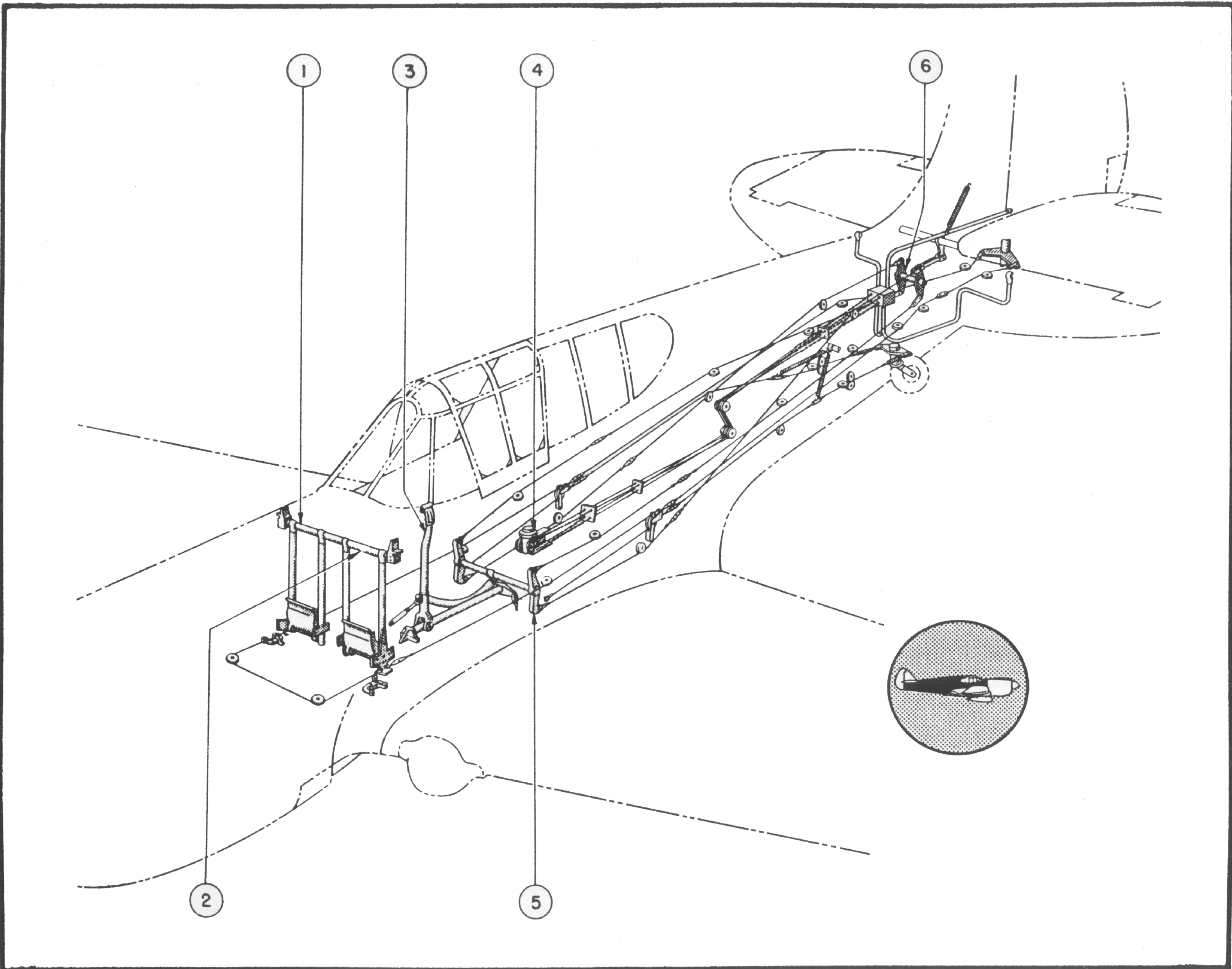
Figure 69—Flight Controls Installation
