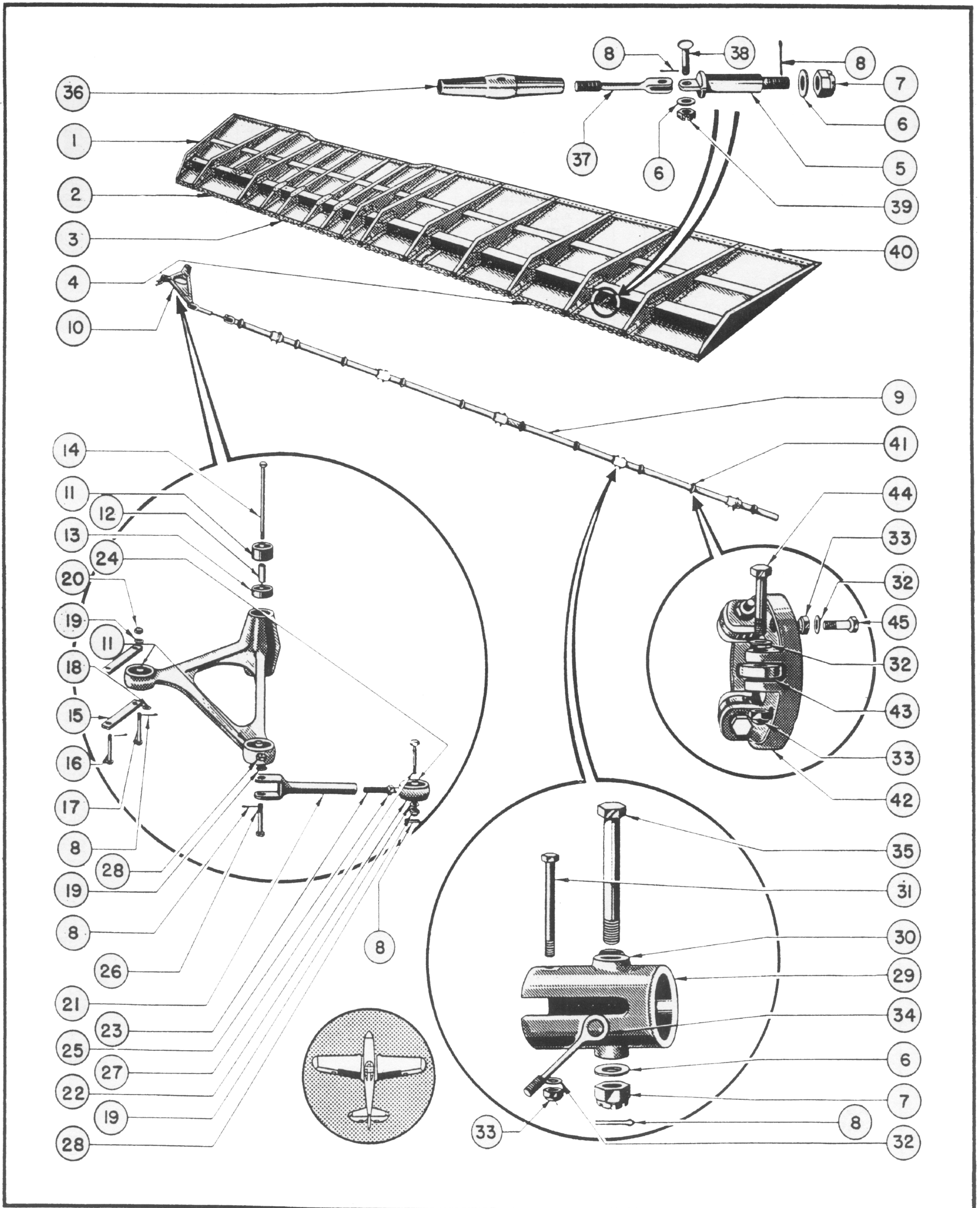
Figure 7—Flap Assembly
