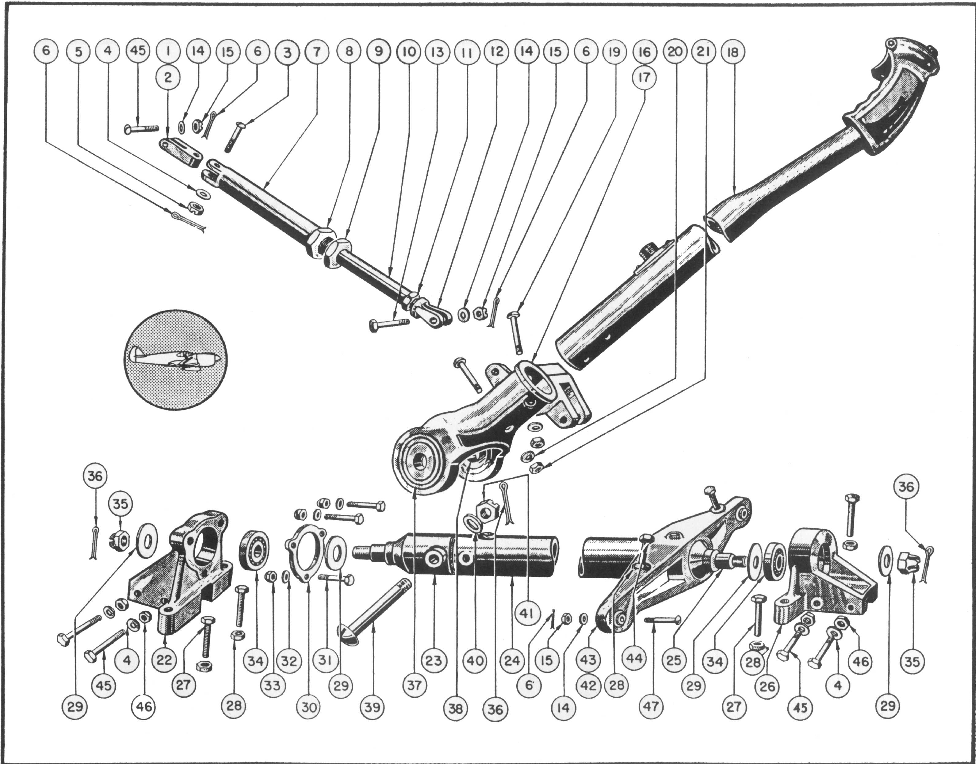
Figure 70—Control Stick and Stop Assembly
