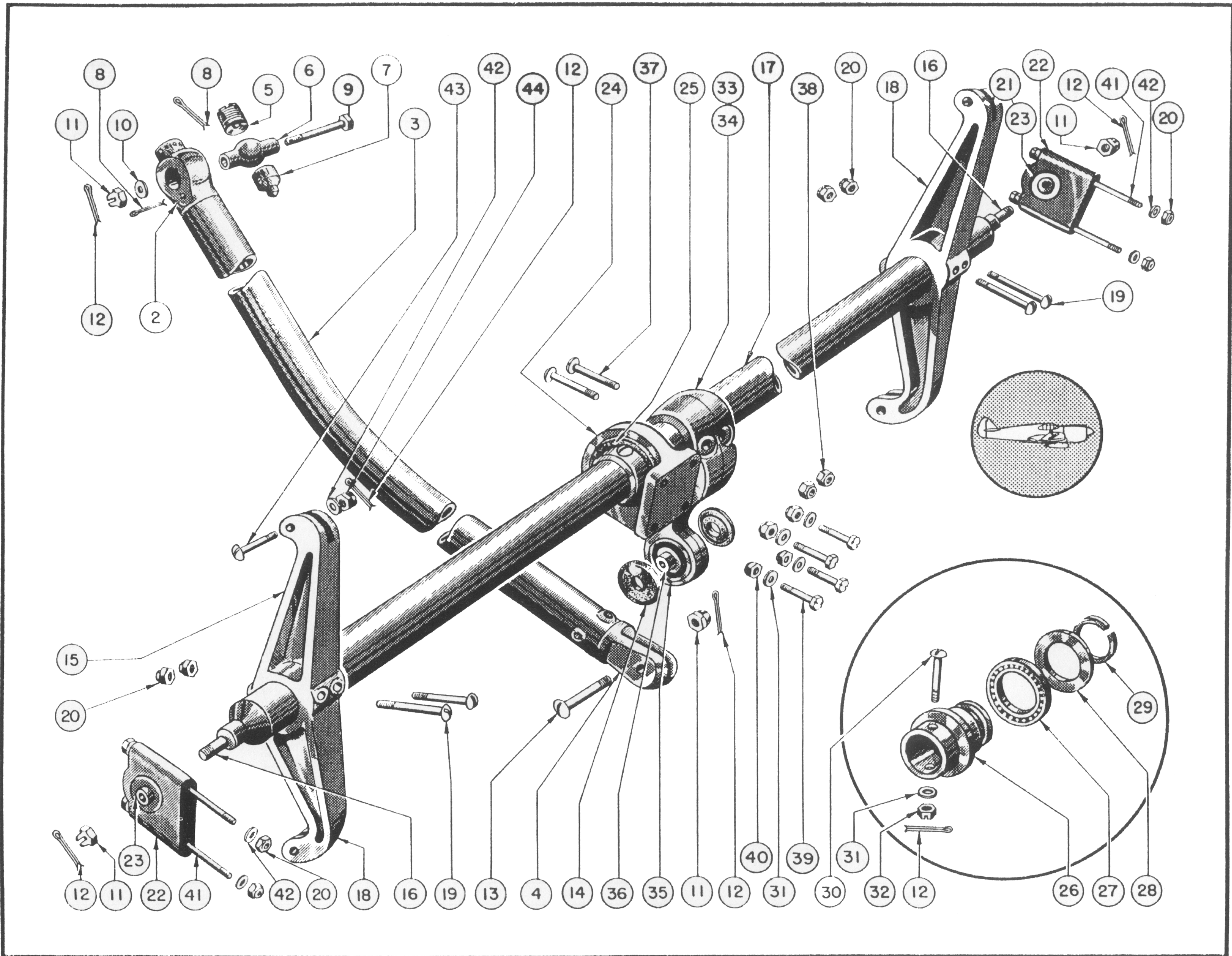
Figure 72—Rod and Jackshaft Assembly
