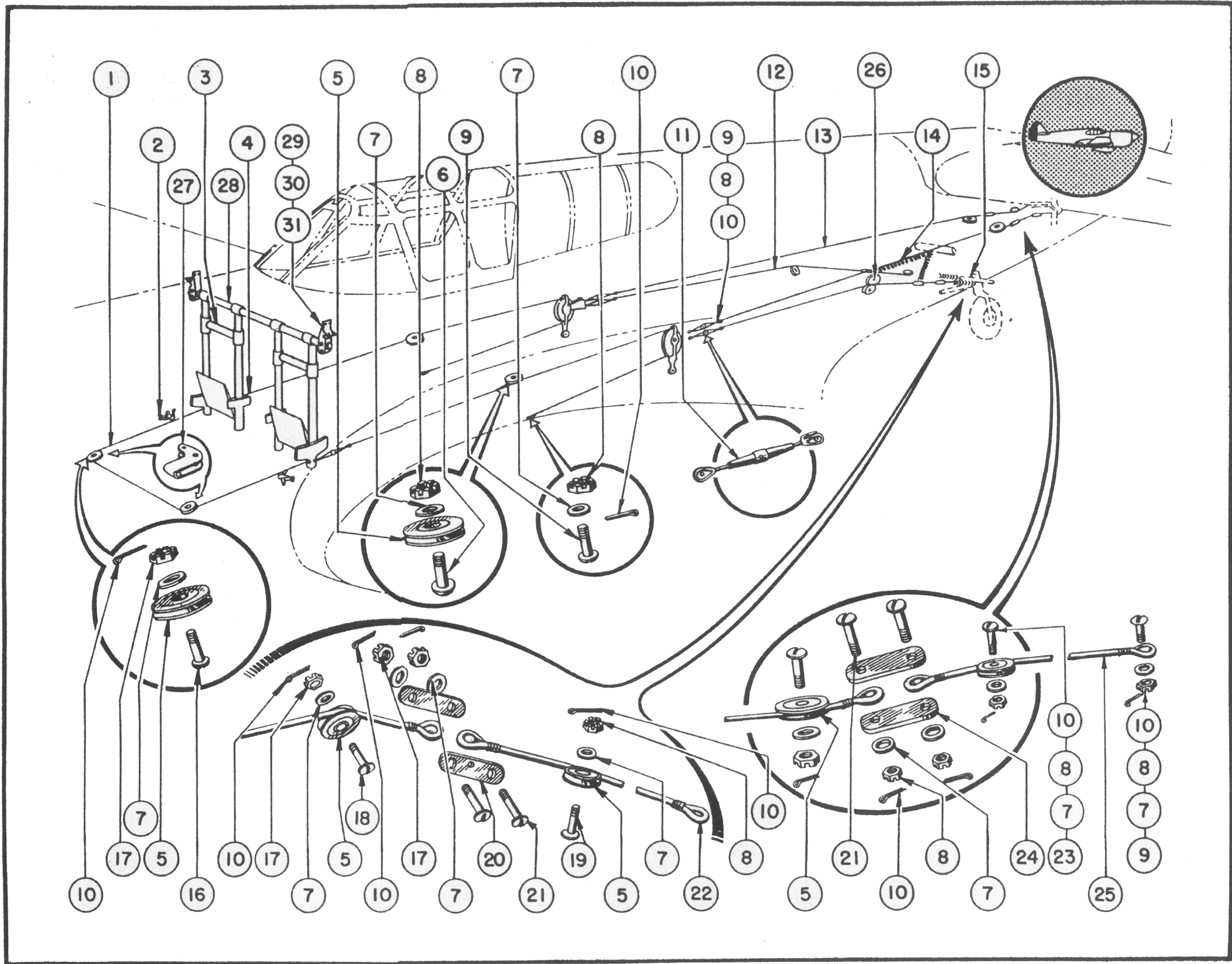
Figure 73—Rudder Controls
