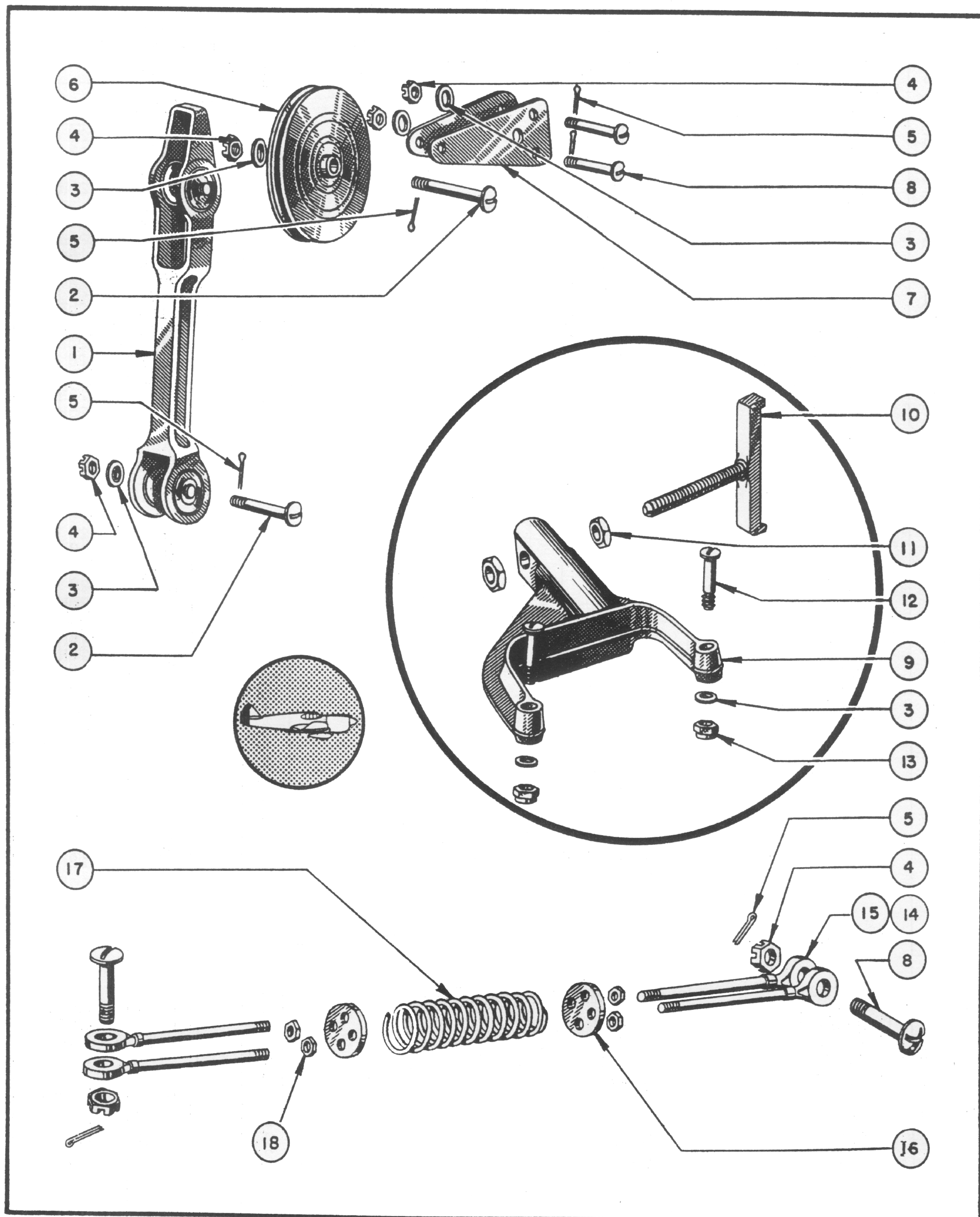
Figure 74—Rudder Control Component Parts
