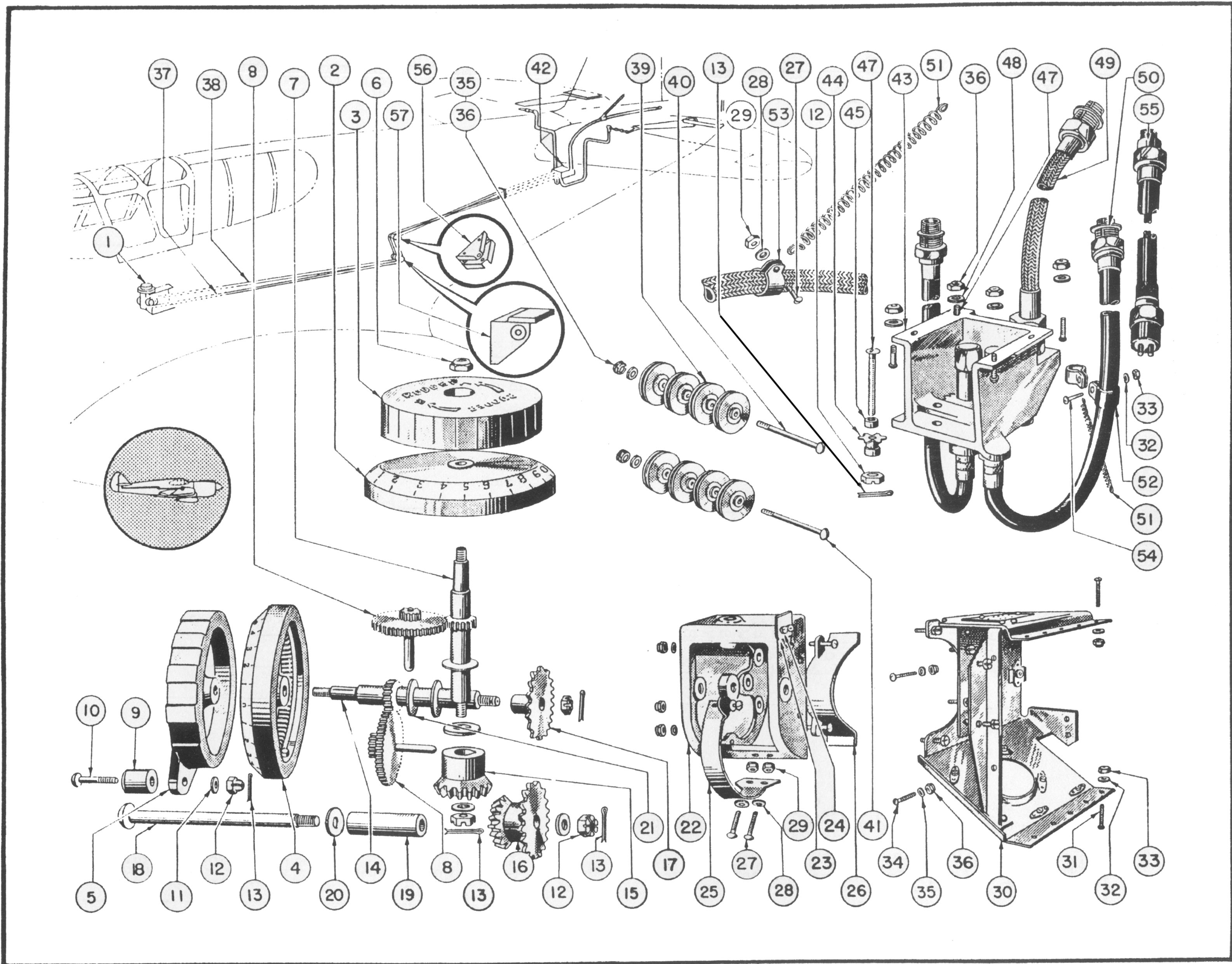
Figure 76—Tab Control Assembly
