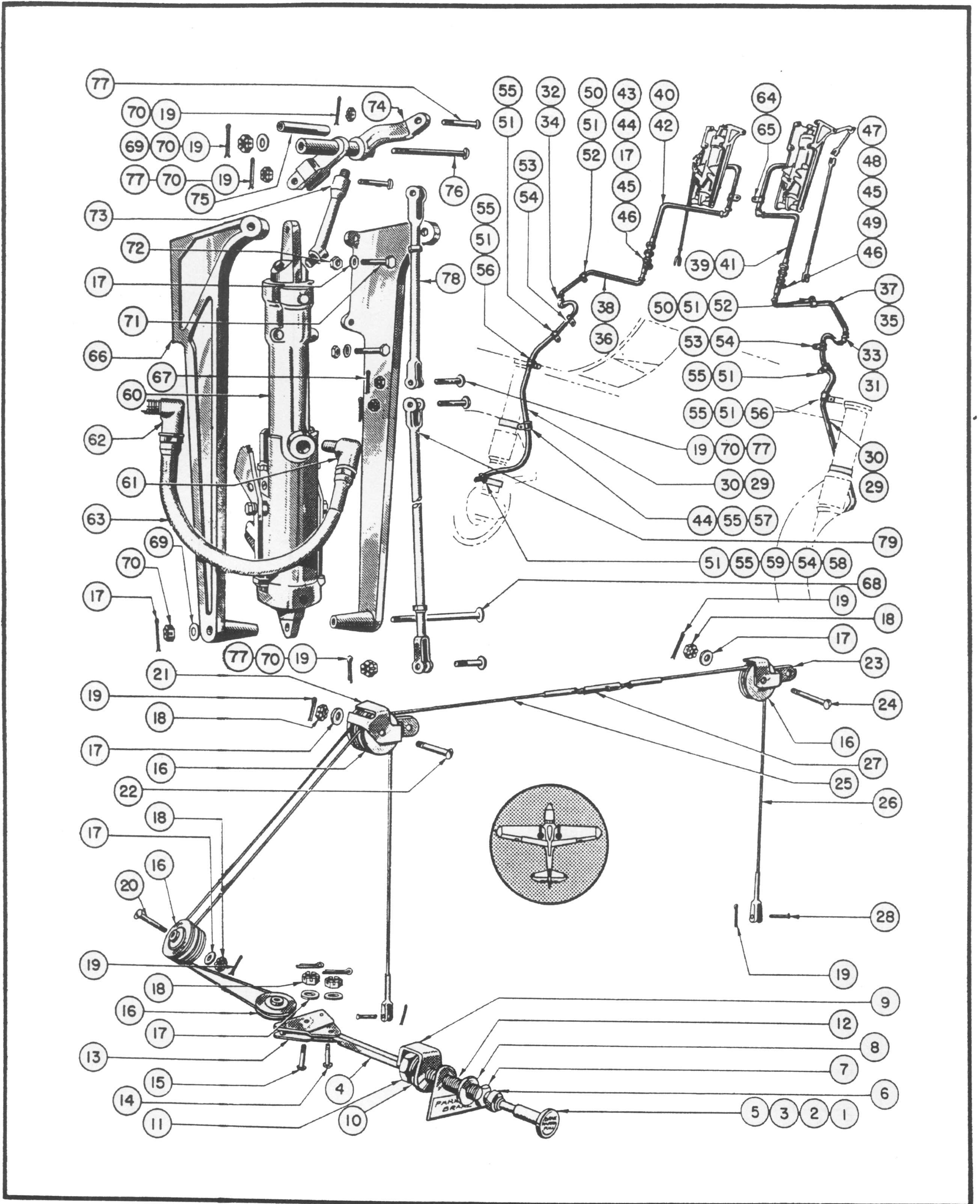
Figure 77—Brake Installation
