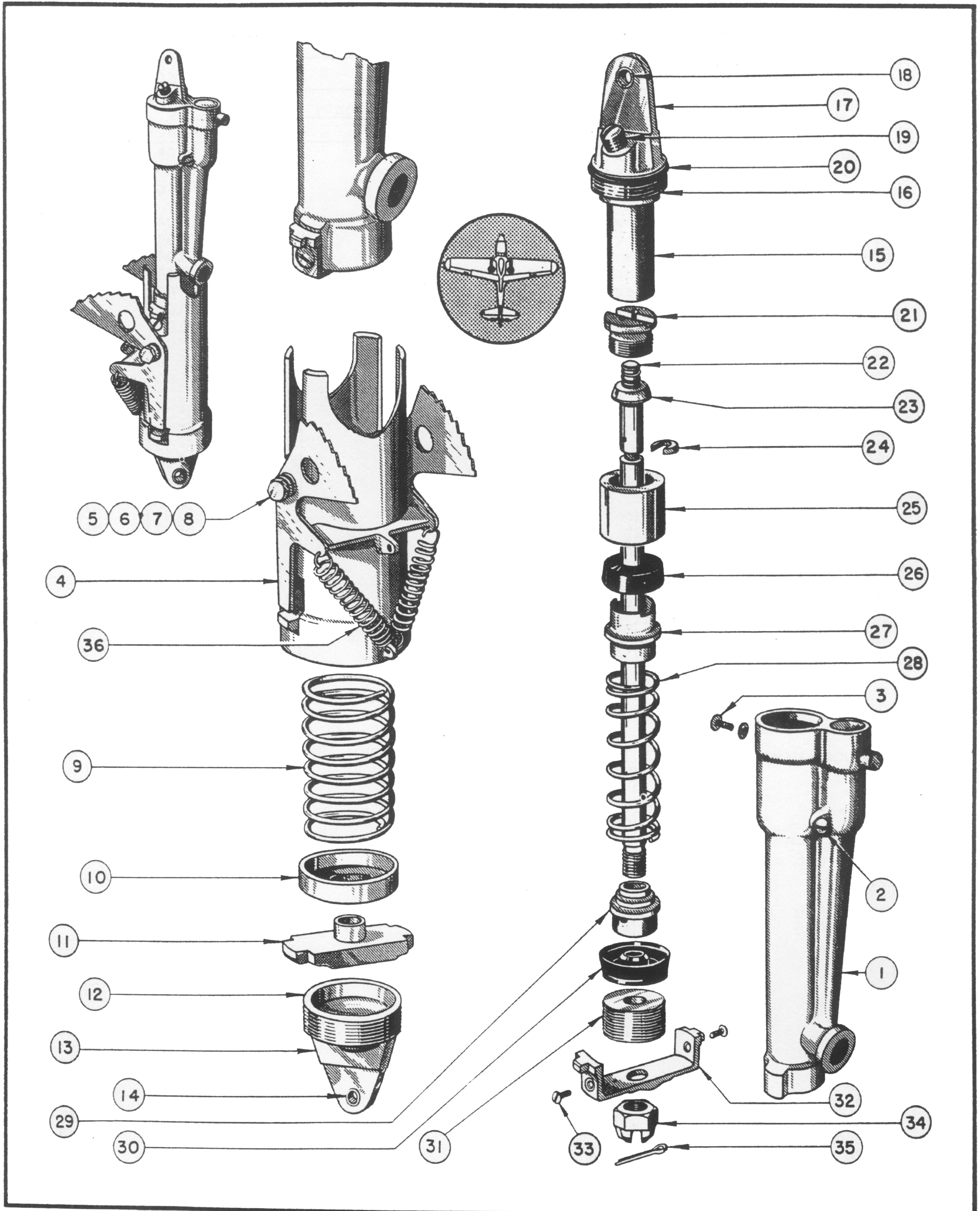
Figure 78—Brake Control Unit
