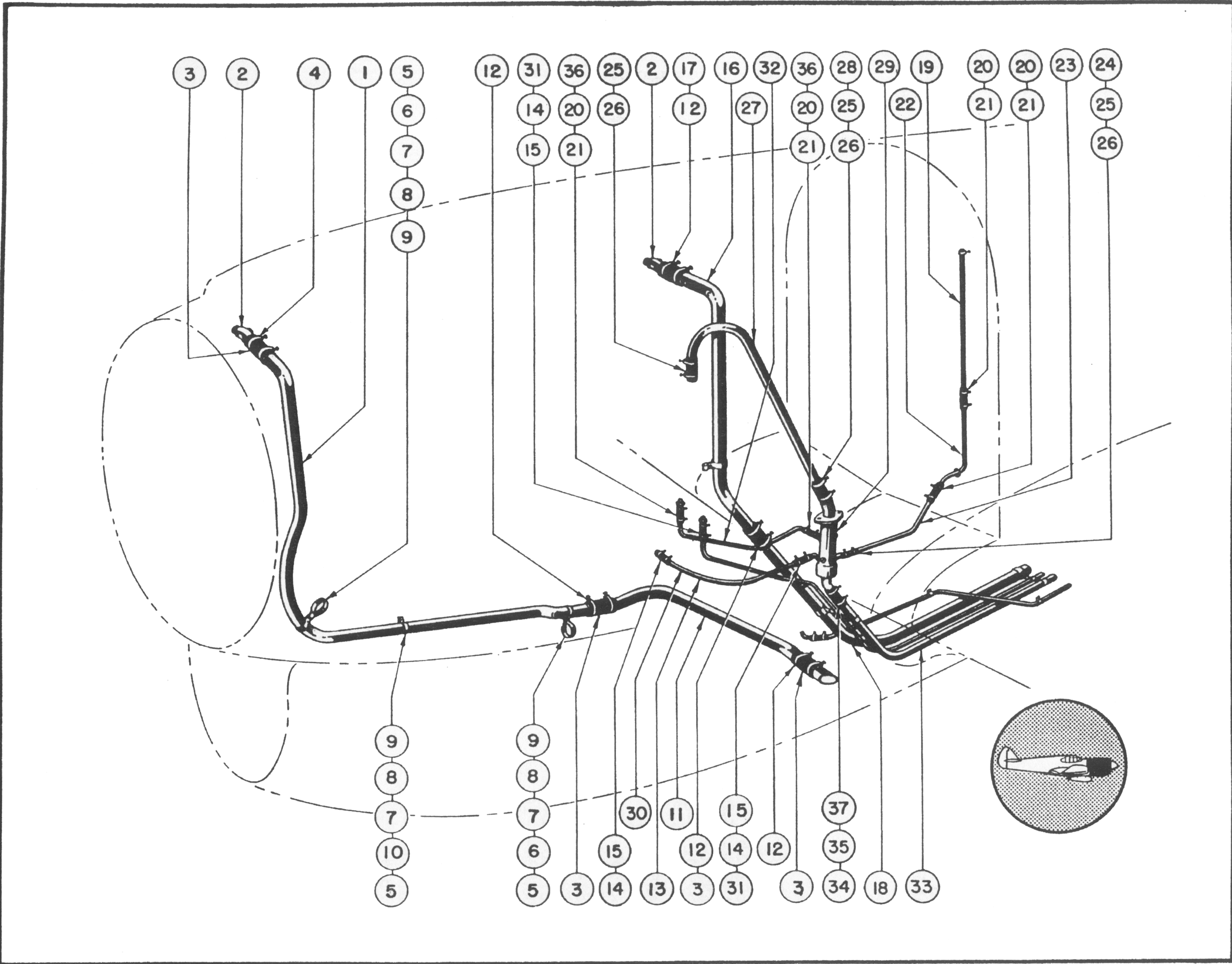
Figure 79—Breather and Vent Installation (A-B)
