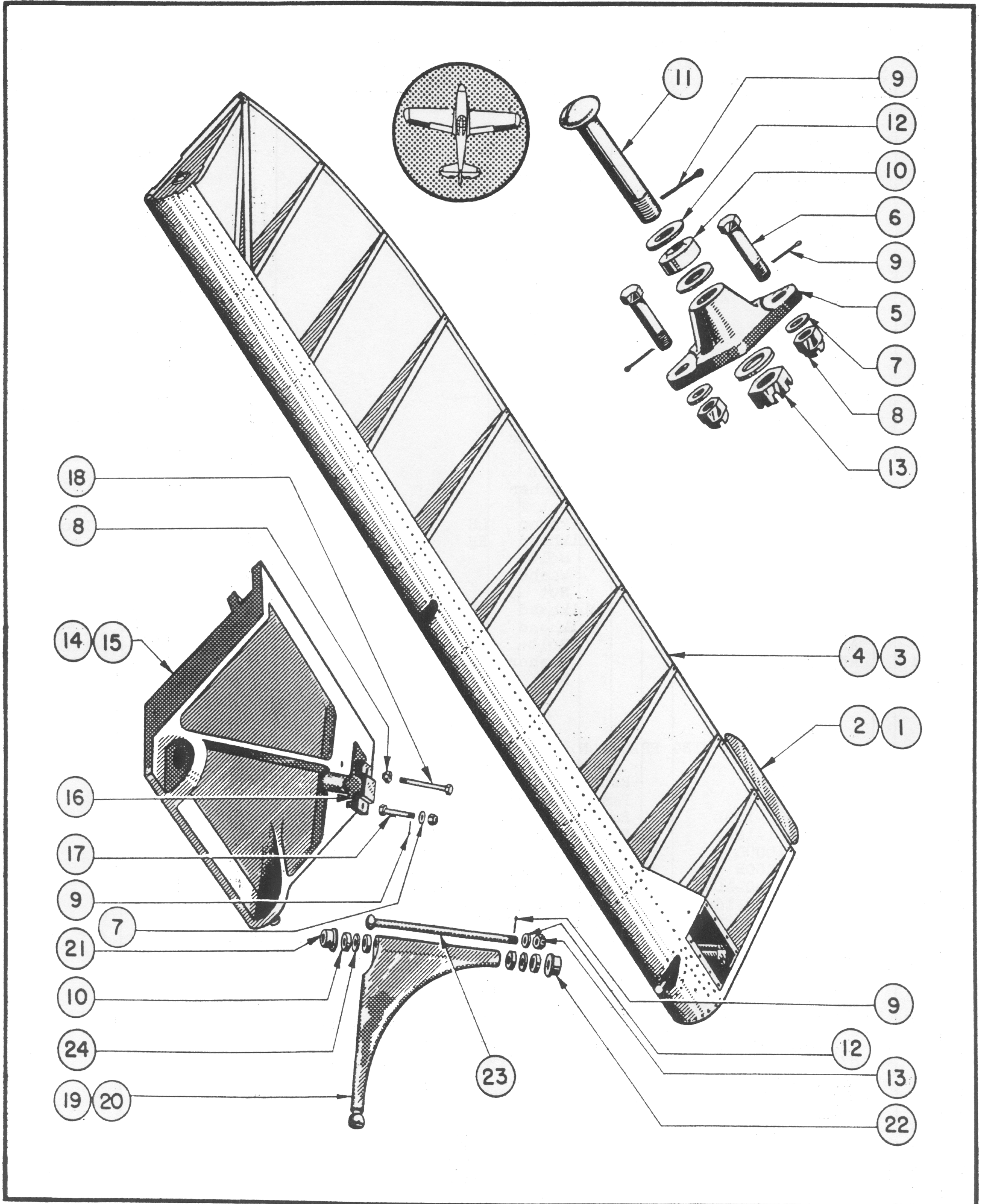
Figure 8—Aileron Assembly
