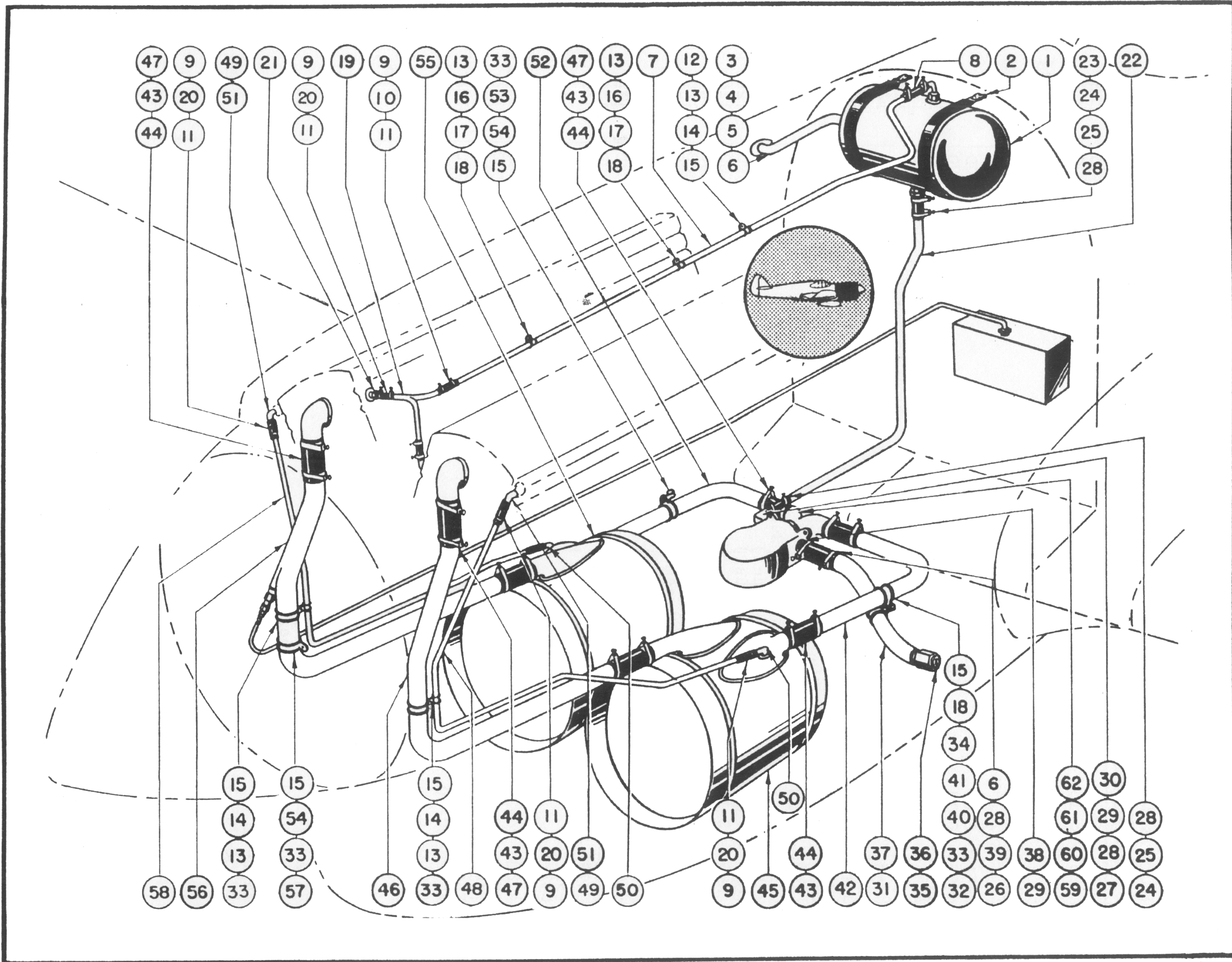
Figure 82—Coolant System (C-W)
