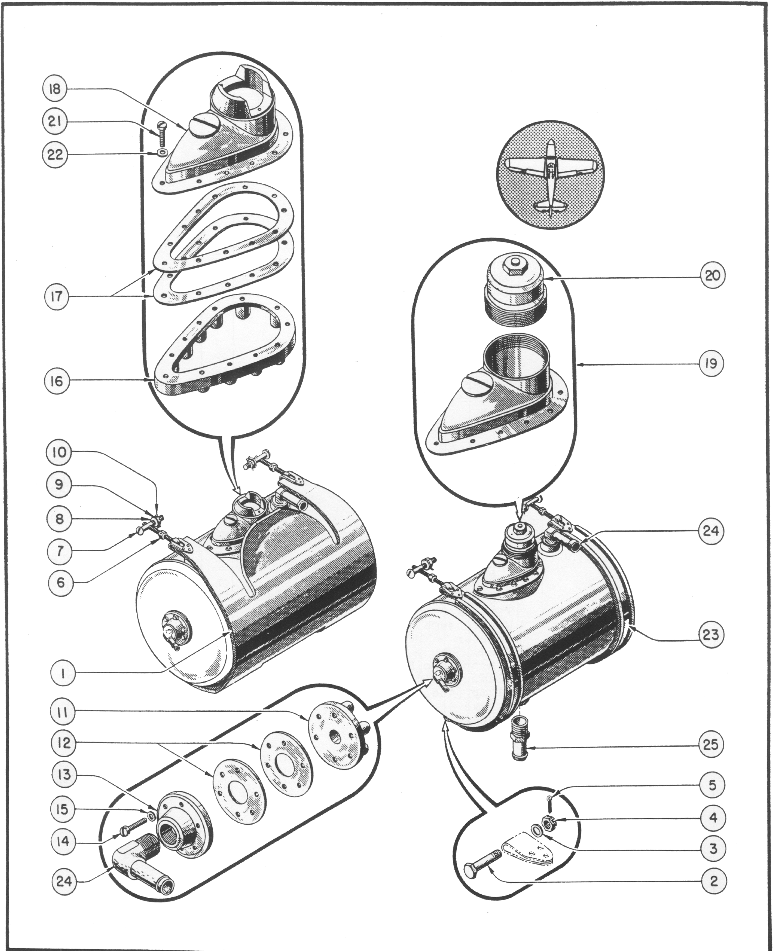
Figure 83—Armor Plating Installation and Coolant Tank Assembly
